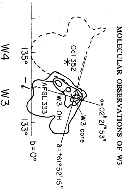
FIG. 1.—Schematic diagram of part of the Perseus spiral arm showing the location of the H II regions W3-4 (dashed outlines) and the associated molecular cloud (solid line). The stars in the OB association Cas OB6 cover the entire area. The center of the open cluster Oc1 352 which excites W4 is marked by an asterisk. The line of constant galactic latitude b = 0^\circ is drawn with tick marks every 1^\circ in galactic longitude, and the central \alpha , \delta axes of the CO observing grid are drawn.
