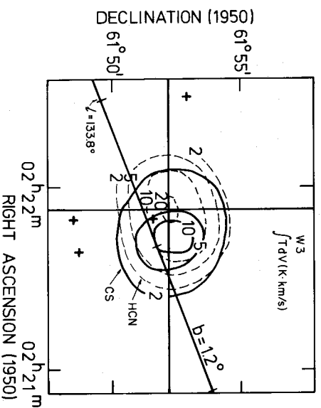
FIG. 9.—Integrated brightnesses \int TdV in \text{K} \cdot \text{km s}^{-1} for CS (solid lines) and HCN (dashed lines).
