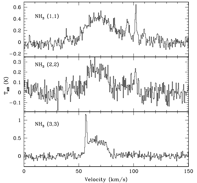
Figure 11. \text{NH}_3 emission spectra towards G23.33-0.30. ( Top ) \text{NH}_3 (1,1) emission showing a broad peak centred at approximately 70 \text{ km s}^{-1} and a line FWHM of approximately 40 \text{ km s}^{-1} . There is a second \text{NH}_3 (1,1) source centred at approximately 102 \text{ km s}^{-1} , with line FWHM of 1.9 \text{ km s}^{-1} . The second source also exhibits hyperfine structure. ( Middle ) \text{NH}_3 (2,2) emission also showing the two features identified in the (1,1) spectrum at a somewhat weaker level. ( Bottom ) \text{NH}_3 (3,3) emission showing a broad emission feature, as for the (1,1) and (2,2) spectra, with peak around 64 \text{ km s}^{-1} and line FWHM approximately 20 \text{ km s}^{-1} . A new narrow-lined feature is seen in the (3,3) spectrum at 56.7 \text{ km s}^{-1} , with a line width of 1.2 \text{ km s}^{-1} . This feature is suspected to be a maser.
