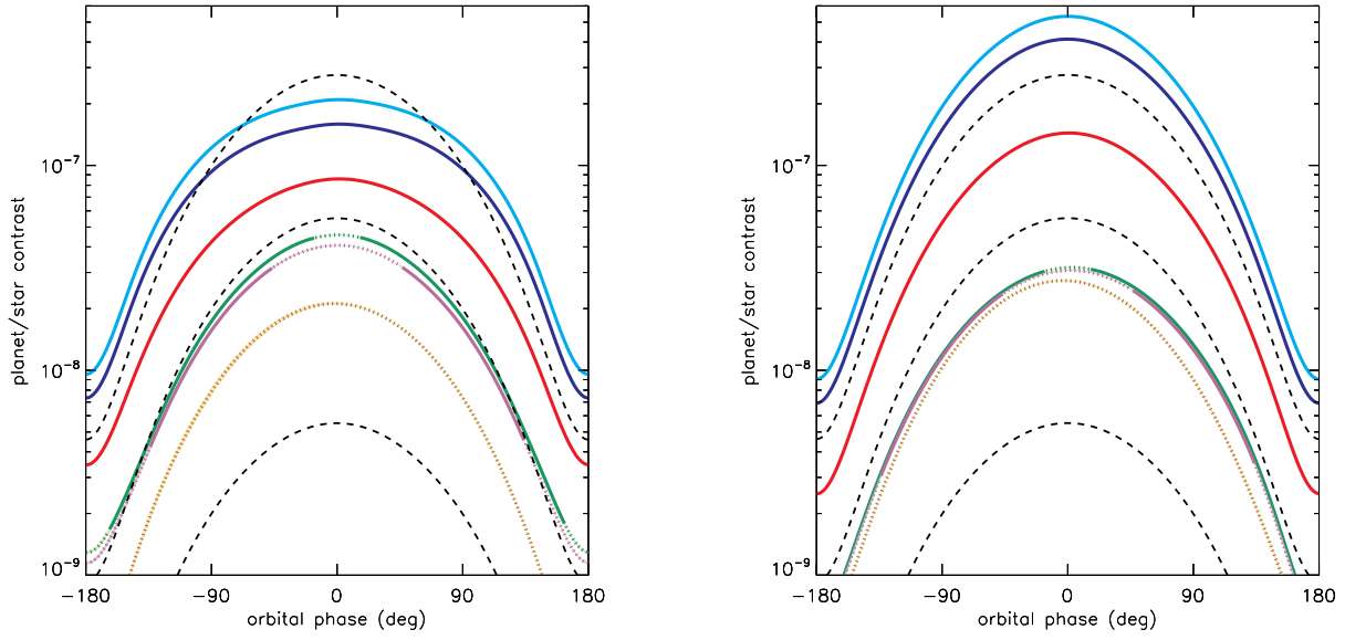
Fig. B.11. Reflection phase curves computed for an aquaplanet with a 10 mbar \text{N}_2 -dominated (+376 ppm of \text{CO}_2 ) atmosphere in synchronous rotation ( left ) and 3:2 spin-orbit resonance ( right ).
