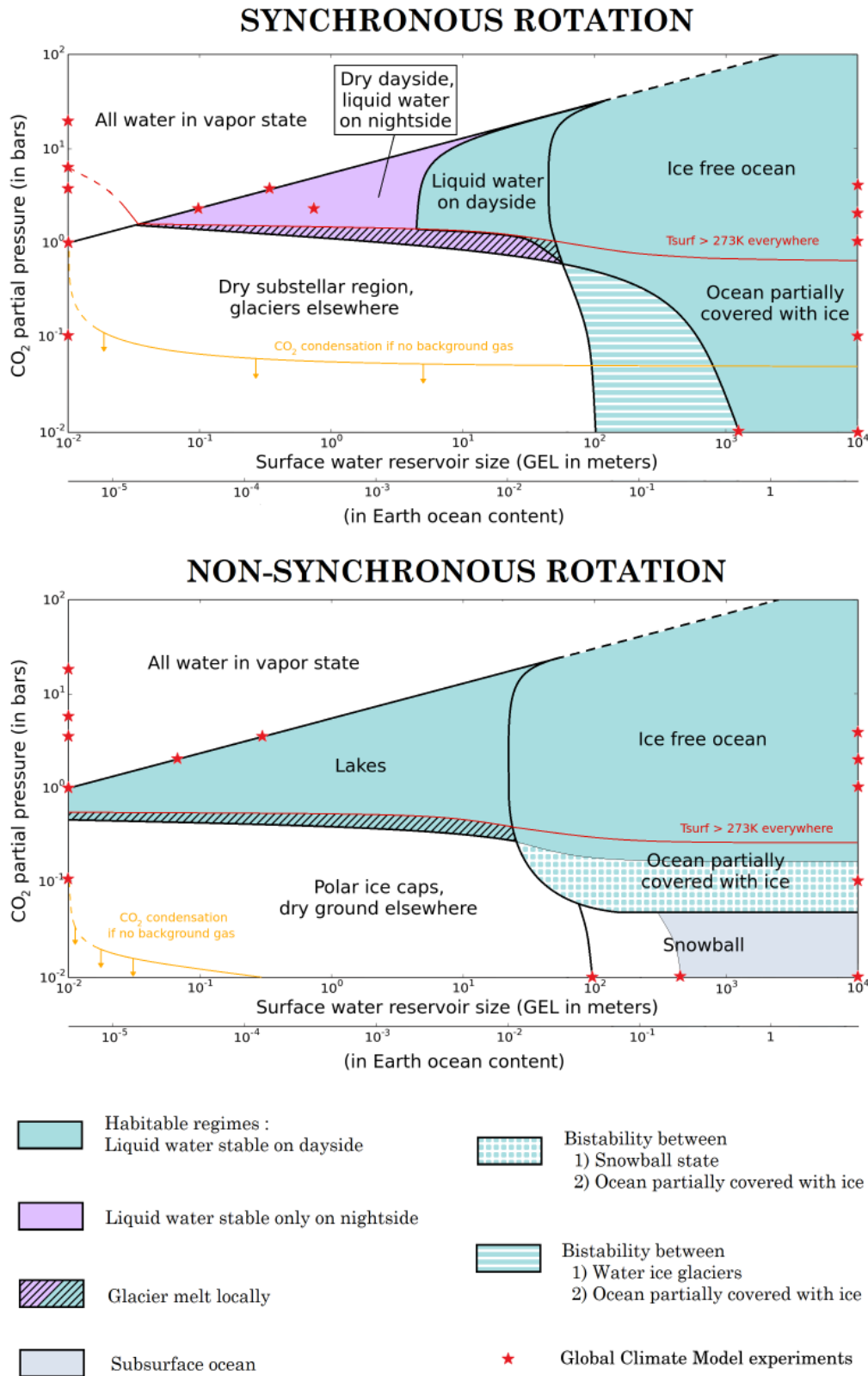
Fig. 1. Schematic diagrams of the possible climate regimes reached as function of the \text{CO}_2 atmospheric content (in bar) and the \text{H}_2\text{O} content available at the surface (in global equivalent layer (GEL), in meters). The top and bottom panels describe the case of synchronous and asynchronous spin states, respectively. The red stars indicate the parts of the diagram that have been probed in this work using GCM simulations. The stars that lie on top of the left y -axis correspond to the case of a dry surface and atmosphere while those on the right y -axis consider planets completely covered by water. The presence of a background gas such as \text{N}_2 could significantly modify the lower part of the diagram ( p\text{CO}_2 < 1 bar typically). It would favor the heat redistribution, which in turn could (1) prevent the \text{CO}_2 atmospheric collapse and (2) reduce the amount of ice possibly trapped in water ice glaciers.
