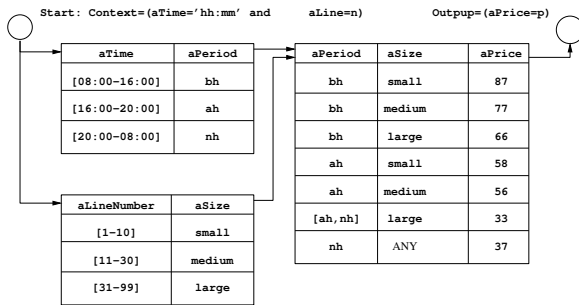
Fig. 4. A simple intuitive example of an XTT system
