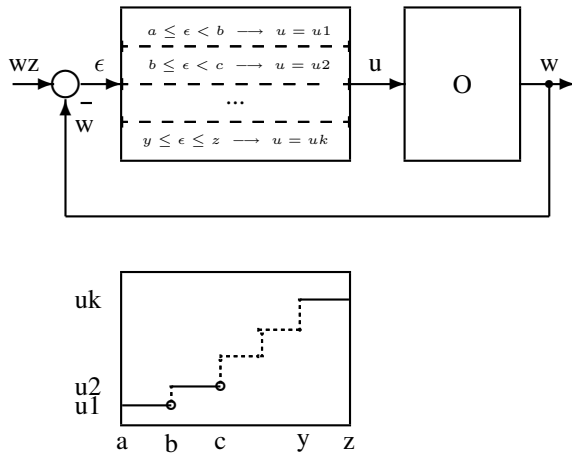
Fig. 1. A simple application of a rule-based system as a direct controller
