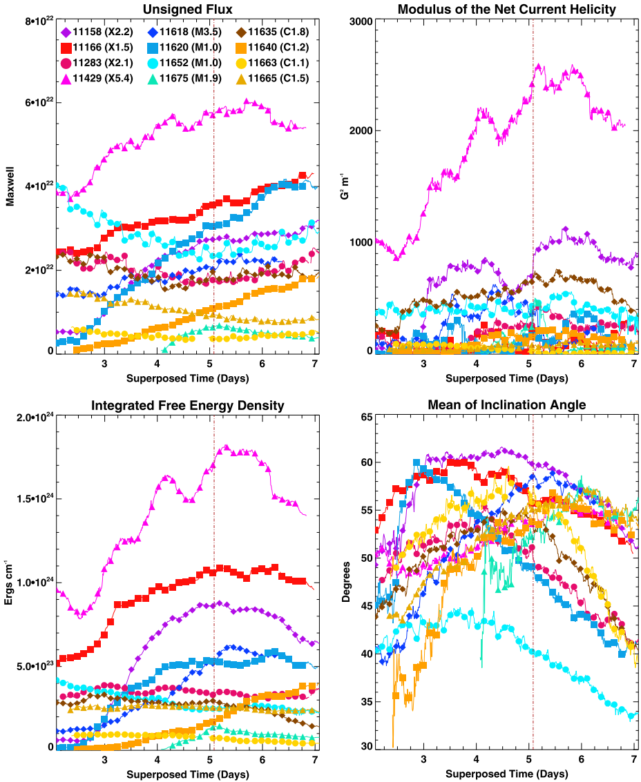
Figure 7 Clockwise from top left, temporal profiles of the total unsigned flux [USFLUX], the modulus of the net current helicity [ABSNJZH], the mean value of the inclination angle [MEANGAM], and the integrated total free-energy density per active region [TOTPOT]. The entire sample is color coded: active regions associated with X-class flares are represented with red-purples, M-class by blue-greens, and C-class by yellow-browns. For clarity a larger symbol is plotted every three hours, i.e. every 15th point. The legend is in the top-left panel. The time profiles are adjusted to align the flare peaks shortly after the start of Day 5, as denoted by the red dotted–dashed line. Error bars are plotted for all points; however, in most cases, they are smaller than the point size. Scatter in the active-region parameters for NOAA AR 11429 for a few points following the flare peak is due to poor data quality following an eclipse: thermal changes in the HMI front window affect the focus. Periodicities in some of the parameters, most prominently in some temporal profiles of unsigned flux, are systematic effects due to the daily variation of the radial velocity of the spacecraft inherent to the geosynchronous orbit.
