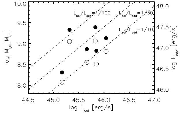
Fig. 5. Black hole mass ( M_{BH} ) vs. bolometric luminosity ( L_{bol} ) for the AGN hosted in the elliptical galaxies. The Eddington luminosity for a given M_{BH} is reported in the right-hand axis. The black hole masses have been estimated from the local L_K - M_{BH} relation (Marconi & Hunt 2003) under two different hypotheses (see 5.2): (1) evolution by a factor of two of the M_{BH}/M_{star} ratio with redshift in comparison to the local values (black filled circles); (2) no evolution of the M_{BH}/M_{star} ratio (empty circles). The three dashed lines represent the loci of L_{bol}/L_{Edd} = 0.01, 0.033 and 0.1 (from left to right).
