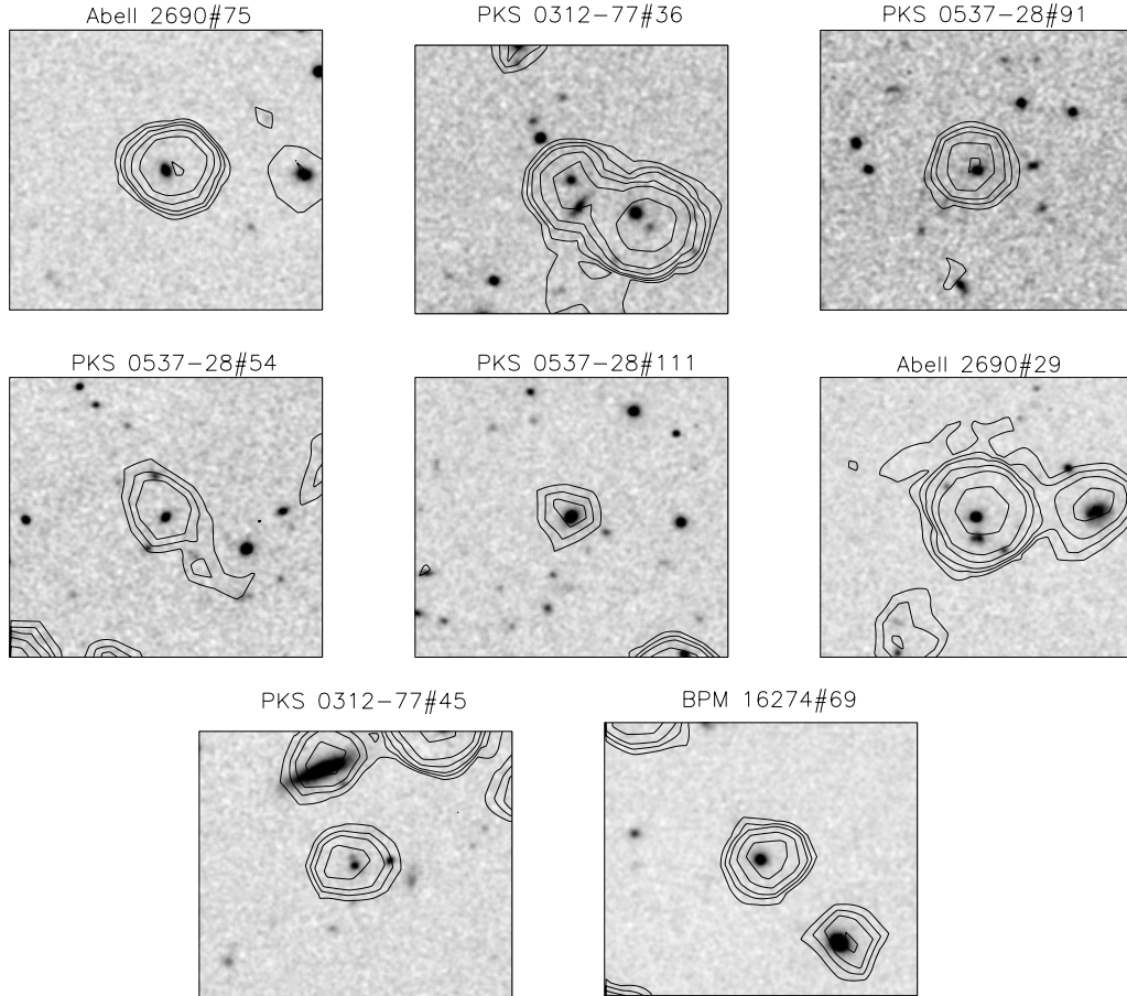
Fig. 1. ISAAC K_s images, centered on the K_s counterpart of the X-ray sources; each box is 30'' wide. North is to the top and East to the left . Contour levels of the 24\ \mu\text{m} emission corresponding to [3, 4, 5, 7, 10, 20, 40]\sigma are superimposed to each image.
