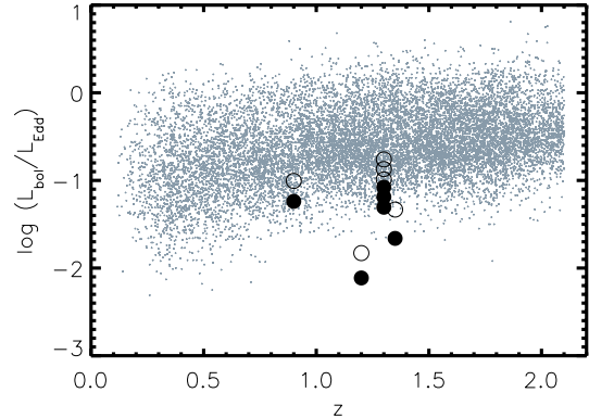
Fig. 6. Bolometric luminosity as a fraction of the Eddington luminosity vs. redshift for the whole sample of SDSS quasars of McLure & Dunlop (2004), plotted as small crosses. The large circles indicate the six HELLAS2XMM AGN hosted in elliptical galaxies (symbols as in Fig. 5).
