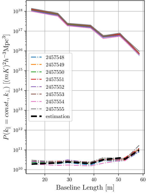
Figure 12. High band power as a function of baseline length for k_{\parallel} = 0 h/Mpc (solid lines) and an average value over the white noise ( |k_{\parallel}| > 1 h/Mpc; dot-dashed lines) for pseudo-Stokes I on each JD of observation. The black dashed line represents estimated power spectrum noise given a system temperature of 2400 K. A very similar relationship obtains for the low band (not shown), but with a higher system temperature of 7000 K. Note that the increase of the noise level with baseline length is correctly modeled, as the compact array has a decreasing number of baselines which are averaged together in a given (k_{\parallel}, k_{\perp}) bin.
