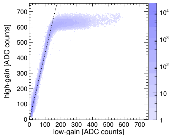
Figure 20. ADC values of the high-gain versus those of the low-gain channel for all 128 strips of a sensor side.
