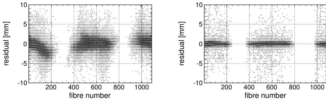
Figure 30. Differences between the hit position in the outer SFT layer calculated from the track parameters and the measured position before (left) and after (right) alignment obtained from a cosmic ray data sample.
