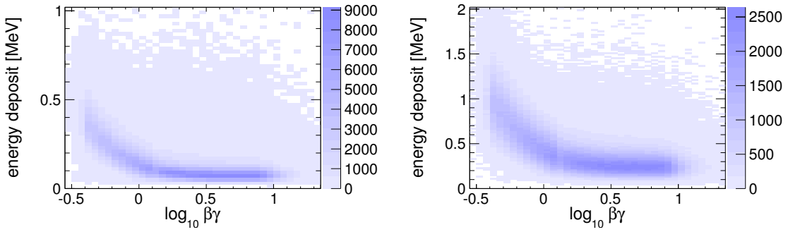
Figure 36. Energy deposit in the inner SSD layer (left) and the inner SFT layer (right) versus \log_{10}(\beta\gamma) for the clean proton and charged pion track sample.
