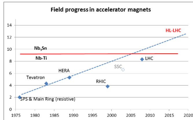
Figure 10: Progress of accelerator magnets for hadron colliders: from 2 to 9 Tesla is the realm of Nb-Ti; beyond 9 Tesla, Nb 3 Sn is needed.
