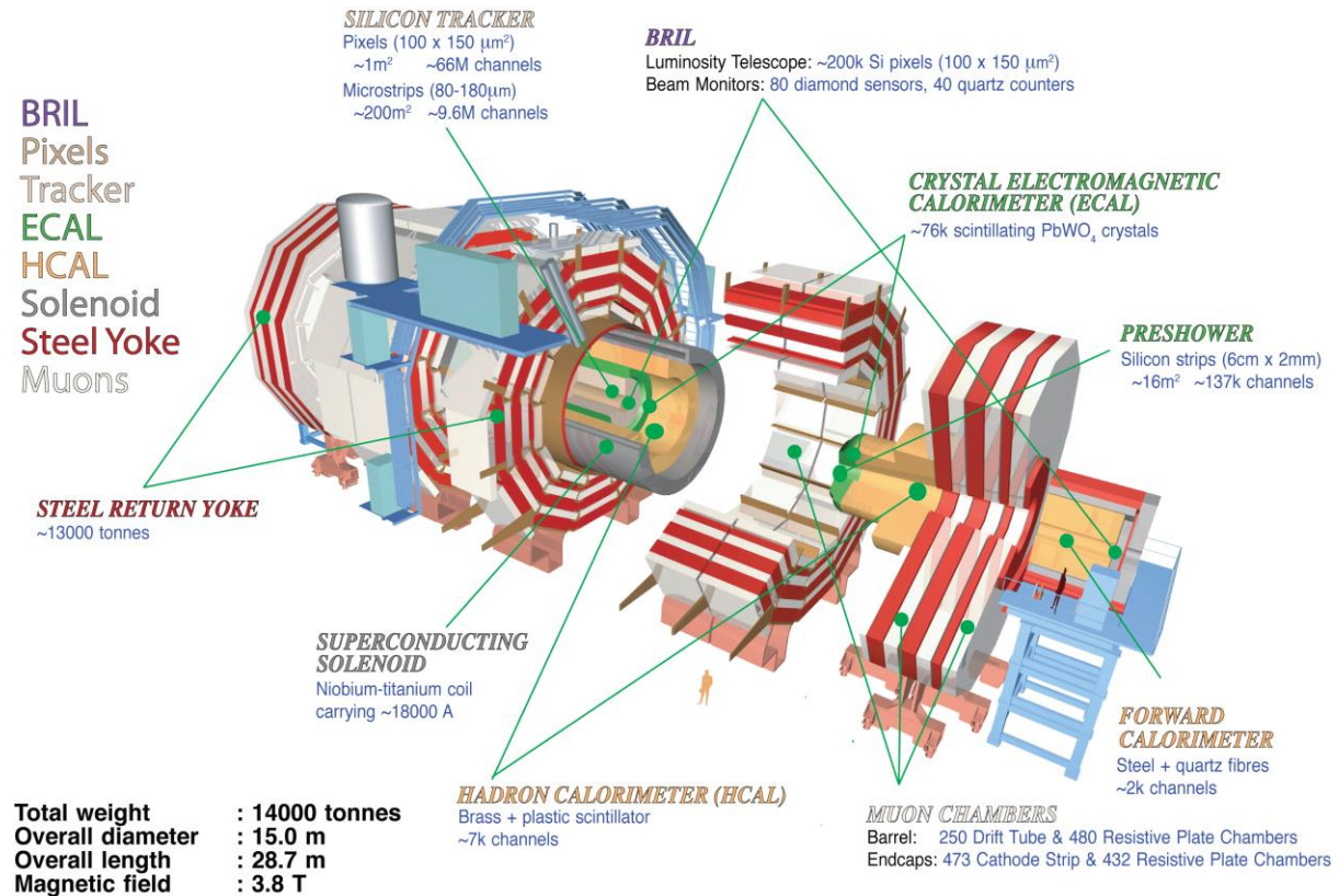
Figure 16: A schematic representation of the CMS Detector in with its various sections in retracted positions. The central yoke block is YBO. The first block (YB+1, and corresponding YB-1) is shown partially moved away from YBO. The second yoke block (YB+2, which has a corresponding YB-2) is shown fully moved past the solenoid vacuum tank. The endcap calorimeters are attached to the first endcap disk YE+1, then endcap CSCs and RPCs, then YE+2, more muon chambers, and YE+3, with additional muon chambers on the front and back. Eventually, another disk, YE+4 will be added at the end to provide shielding from beam related backgrounds. This configuration is repeated on the other end. In operation the detector is closed by moving all pieces together.
