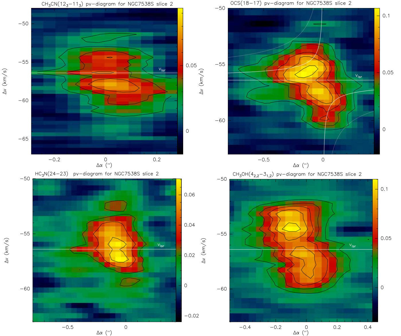
Fig. 10. Position velocity cuts through NGC 7538S mm2 in several lines as marked in each panel along the axis shown in Fig. 8, respectively. The v_{\text{lsr}} is marked. The full and dotted lines in the OCS panel correspond to Keplerian rotation curves around a 1 and 10 M_{\odot} star, respectively. The units of the wedges are \text{Jy beam}^{-1} .
