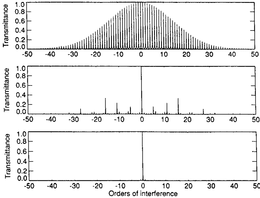
Fig. 2. Illustration of how multiple etalon change the instrument function. (a) Single etalon with a 1 cm gap and 0.8 nm wide interference filter. (b) Same as (a) but with a second etalon with a 0.186 cm gap. (c) Same as (b) but with a third etalon with a 0.025 cm gap.
