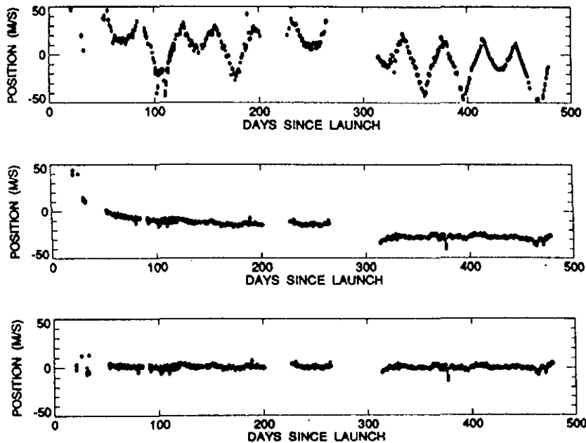
Fig. 7. (a) Position on the HRDI detector in velocity units of the neon calibration line at 14427\text{ cm}^{-1} . (b) Position of the calibration line after correction for the temperature sensitivity of the instrument, leaving a residual long term drift. (c) Position of the calibration line corrected for temperature effects and the long term drift. These same corrections are applied to the HRDI atmospheric observations.
