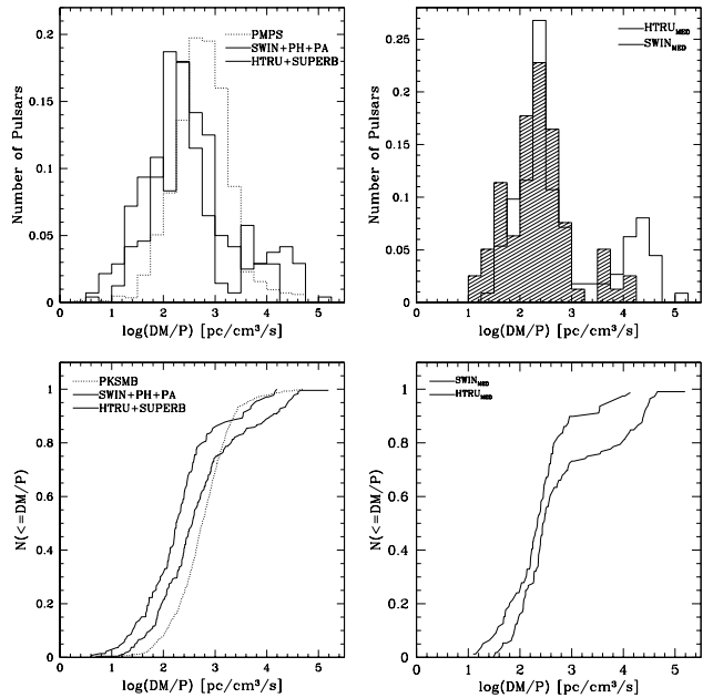
Figure 9. Normalised histograms (top) and cumulative distributions (bottom) of DM/P for Parkes survey discoveries. Left: the dotted curve is for the galactic plane multibeam-survey PMPS (Manchester et al. 2001), with a 3-MHz frequency resolution and a 250 \mu\text{s} time resolution; the solid thin curve is for surveys with the same frequency resolution, but 2\times finer time resolution (SWIN, Edwards et al. 2001; Jacoby et al. 2009; PH, Burgay et al. 2006 and PA, Burgay et al. 2013); the solid thick curve is for the most recent surveys using the BPSR digital backend, with 0.39-MHz frequency resolution and 64 \mu\text{s} time resolution (HTRU, Keith et al. 2010 and SUPERB, Keane et al. 2018). Right: comparison of intermediate-latitude Parkes surveys only. The shaded histogram is for the SWIN surveys, the thick solid line for HTRU-med.
