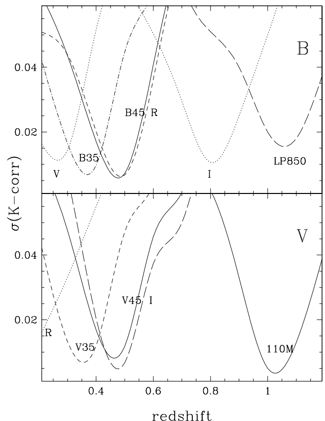
FIG. 2.—Uncertainty in transforming to rest frame ( upper panel ) B and ( lower panel ) V as a function of redshift for V , R_C , and I_C , HST 850LP (WFPC) and 110M (NICMOS), and the B35 , V35 , B45 , and V45 filters described in the Appendix.
