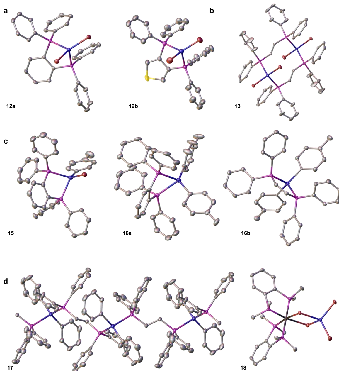
Figure 6. Single crystal X-ray structures of Zn(II)-diphosphine adducts. a , Mononuclear complexes [\text{ZnBr}_2(\text{PP})] , PP = dpbz ( 12a ) and dpth ( 12b ). Analogous structures with sciopp ( 12c ); iPrDuPhos ( 12d ); cis -dppen ( 12e ); dppp ( 12f ); norphos ( 12g ) and dmbz ( 12h ) are shown in Supplementary Figures 91, 95, 99, 103, 107 and 111 respectively. b , Dinuclear complex [\{\text{ZnBr}_2(\mu\text{-trans-dppen})\}_2] , 13 . c , Diphosphine monorarylzinc adduct [\text{ZnBr}(4\text{-tolyl})(\text{dpbz})] ( 15 ) and diarylzinc adducts [\text{Zn}(\text{Ar})_2(\text{PP})] 16a (PP = dpbz, Ar = 4-tolyl) and 16b (PP = cis -dppen, Ar = 4-tolyl); analogous structure of 16c (PP = dppp, Ar = Ph) is shown in Supplementary Figure 137. d , Polymeric diarylzinc adduct [\{\text{ZnPh}_2(\mu^2\text{-dppe})\}_n] 17 . e , Mixed Fe-Zn complex [(\text{dmbz})_2\text{Fe}(\mu\text{-Br})_2\text{ZnBr}_2] , 18 . Thermal ellipsoids set at 50% probability, hydrogen atoms and any solvents of crystallisations omitted for clarity.
