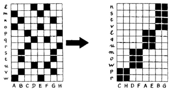
Figure 4. Permutated matrix display from Bertin (1967). This figure was devised to illustrate the possibility of sorting a matrix to reveal block-diagonal structure.
