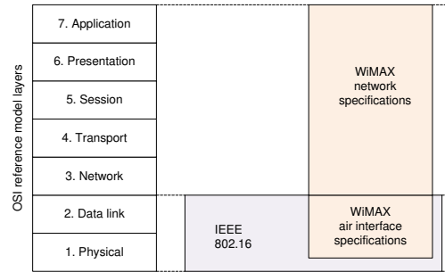
Fig. 7. Relationship between IEEE 802.16 and WiMAX, with respect to the OSI reference model [19].
