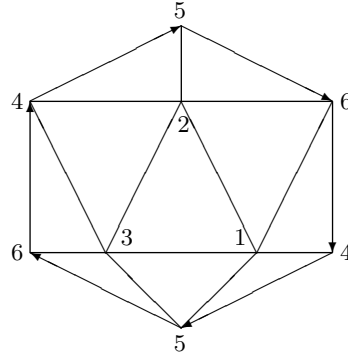
FIGURE 1. 6-vertex triangulation of \mathbb{R}P^2 .
