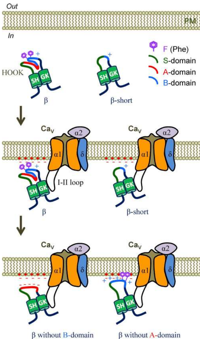
Figure 9. Schematic model of \beta subunit HOOK region-mediated regulation of \text{Ca}_V channels. In the absence of the \alpha 1 subunit, the \beta or \beta -short forms bind membrane phospholipids too weakly to direct stable membrane association on their own (top). They are localized in the cytosol in cells without an \alpha 1 subunit. In the presence of the \alpha 1 subunit (middle), they can be recruited to the plasma membrane through the cooperative interaction between GK domain and I-II loop, and the polyacidic (A) and polybasic (B) domains of the HOOK region may partially associate each other; thus, the HOOK region of the \beta subunit looks charged as weak positive with two hydrophobic Phe residues. Therefore, the HOOK region may interact with the anionic membrane phospholipids through electrostatic forces. The HOOK region of the \beta -short subunit does not have an A domain but contains three basic amino acids without Phe residues. The HOOK region of the \beta -short subunit is also charged as positive and can interact with the plasma membrane. When the B domain was deleted from \beta subunit (bottom), HOOK becomes acidic and cannot interact with the anionic membrane phospholipids. The dissociation of the \beta subunit HOOK region from the plasma membrane promotes the inactivation of \text{Ca}_V currents and augments the \text{PIP}_2 sensitivity of \text{Ca}_V channels like the cytosolic \beta subunits. In contrast, when the A domain was deleted from the \beta subunit, the HOOK region becomes more positive, can directly associate with the plasma membrane, and enhances
