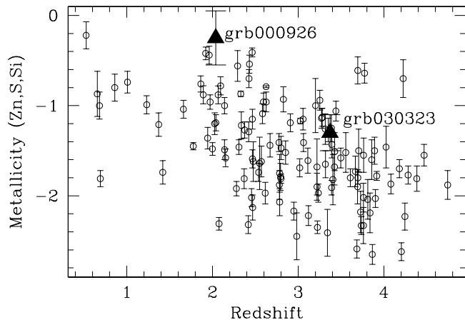
Fig. 6. Comparison of the metallicities of a sample of QSO-DLAs, taken from Prochaska et al. (2003a) (open circles), with the two GRBs for which a metallicity has been determined (solid triangles): GRB 000926 and GRB 030323 (this paper). The GRB hosts are located at the metal-rich end of the QSO-DLA distribution.
