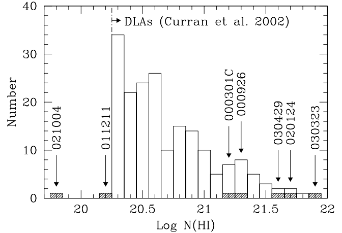
Fig. 4. Histogram of the column densities of DLA systems measured through the damping wings of Ly \alpha discovered in the spectrum of a background QSO (compilation taken from Curran et al. 2002). The shaded histogram shows measurements in GRBs for which the redshift was large enough to detect Ly \alpha . Out of 7 GRBs, 5 show neutral hydrogen column densities above the DLA definition of 2 \times 10^{20} atoms \text{cm}^{-2} ( \log N(\text{H I}) = 20.3 ). The host of GRB 030323 contains a column density larger than in any observed (GRB- or QSO-) DLA system.
