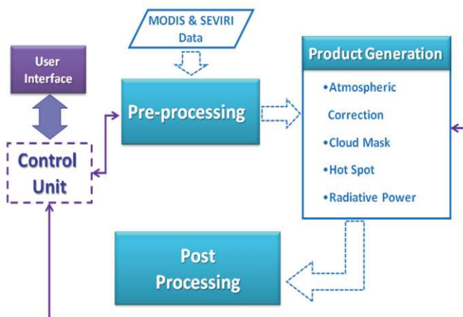
Figure 1. Scheme of the HOTSAT volcano monitoring system.
