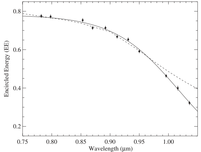
Figure 10. Wavelength vs. encircled energy (EE) fraction for a 3 pixel aperture. The solid line is a fit (Equation (A1)) to the measured data points. The dotted line is the relation from Sirianni et al. (2005).
