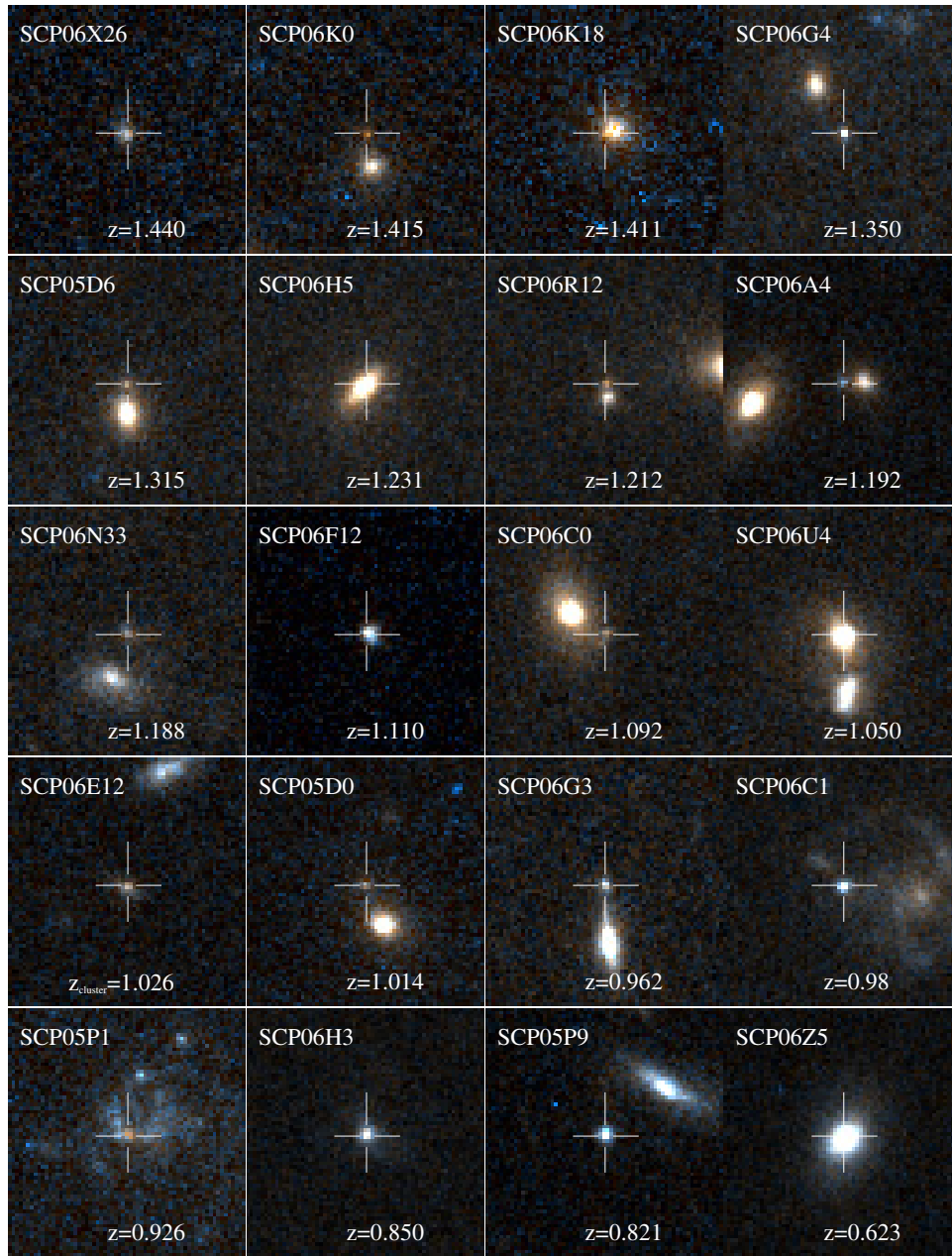
Figure 1. Composite color ( i_{775} and z_{850} ) images of 20 SNe Ia from the HST Cluster Supernova Survey. Each SN Ia is shown in a box of 3''.2 \times 3''.3 (north is up and east is left). Note that the redshift of SCP06E12 is uncertain, and we use the cluster redshift as a guide.
