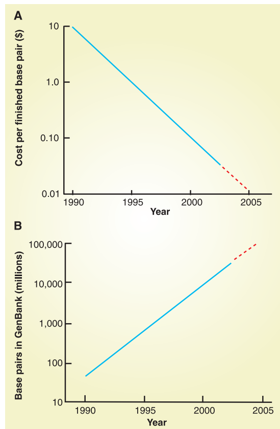
Fig. 1. (A) Decrease in sequencing costs, 1990–2005. (B) Increase in DNA sequence in GenBank, 1990–2005.
