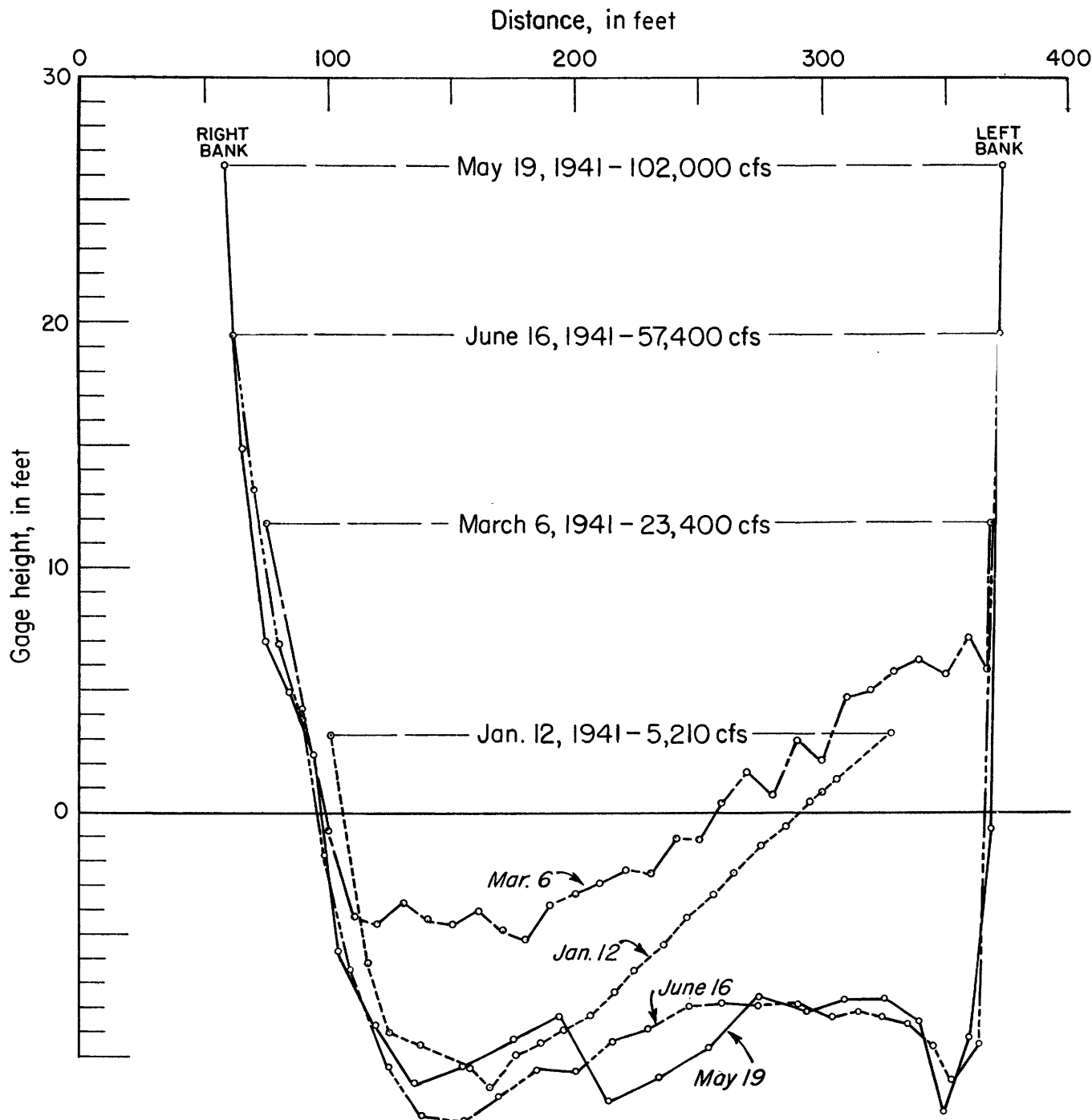
FIGURE 24.—Channel cross sections during progress of flood, December 1940-June 1941, Colorado River at Grand Canyon, Ariz.
