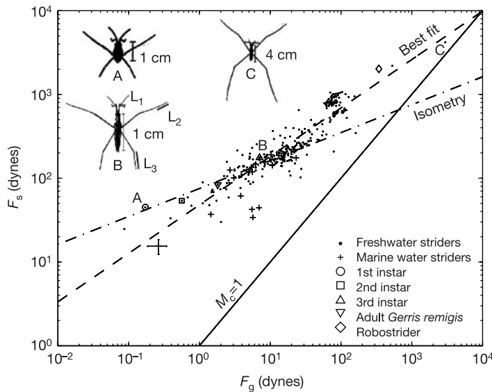
Figure 2 The relation between maximum curvature force F_s = \sigma P and body weight F_g = Mg for 342 species of water striders. \sigma is the surface tension of either pond water ( 67 \text{ dynes cm}^{-1} ) or sea water 17 ( 78 \text{ dynes cm}^{-1} ) at 14^\circ\text{C} and P = 4(L_1 + L_2 + L_3) is twice the combined lengths of the tarsal segments (see strider B). Anatomical measurements were compiled from existing data 20,26–29 . Open symbols denote striders observed in our laboratory. Insets show the adult Gerris remigis (B) and extremes in size: the first-instar infant Gerris remigis (A) and the Gigantometra gigas 20 (C). The solid line
