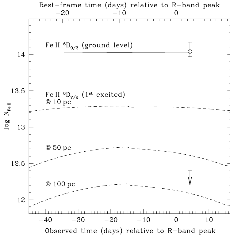
Fig. 7.— Expected population of the first excited level of Fe II ( {}^6D_{7/2} , indicated with the dashed lines) due to excitation by UV photons released by iPTF 13ajg, if the Fe II atoms were located at a distance of 10 pc, 50 pc, and 100 pc from the UV source. The upper limit on the column density, \log N(\text{Fe II } {}^6D_{7/2}) < 12.4 , shows that the Fe II atoms (as detected by the narrow absorption lines) are at least 50 pc away from iPTF 13ajg.
