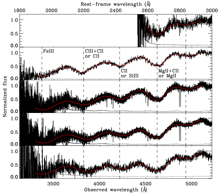
Fig. 4.— The blue side of the spectra taken at epochs 1–5 or phase -9 , -8 , -4 , +8 , and +10 days (top to bottom panels), normalized by the blackbody fits (see Fig. 3), are shown by the black solid lines. The spectra have not been smoothed. The corresponding error spectra are indicated with the dotted lines. Gaussian fits are shown by the solid red lines. To illustrate the evolution of the central wavelength of the lines with time, their best-fit wavelengths in the earliest epoch are marked with the vertical dashed lines. The strengths of these features evolve little to moderately over the course of 20 rest-frame days. The epoch 3 and 4 X-shooter spectra clearly display the narrow absorption features of Mg II and Fe II between 4000 \text{ \AA} and 5000 \text{ \AA} (observed); these are less significant at the other epochs owing to the lower spectral resolution. In the second panel from the top we list the line identification of the broad features according to Howell et al. (2013) (top label) and Quimby et al. (2011) (bottom label).
