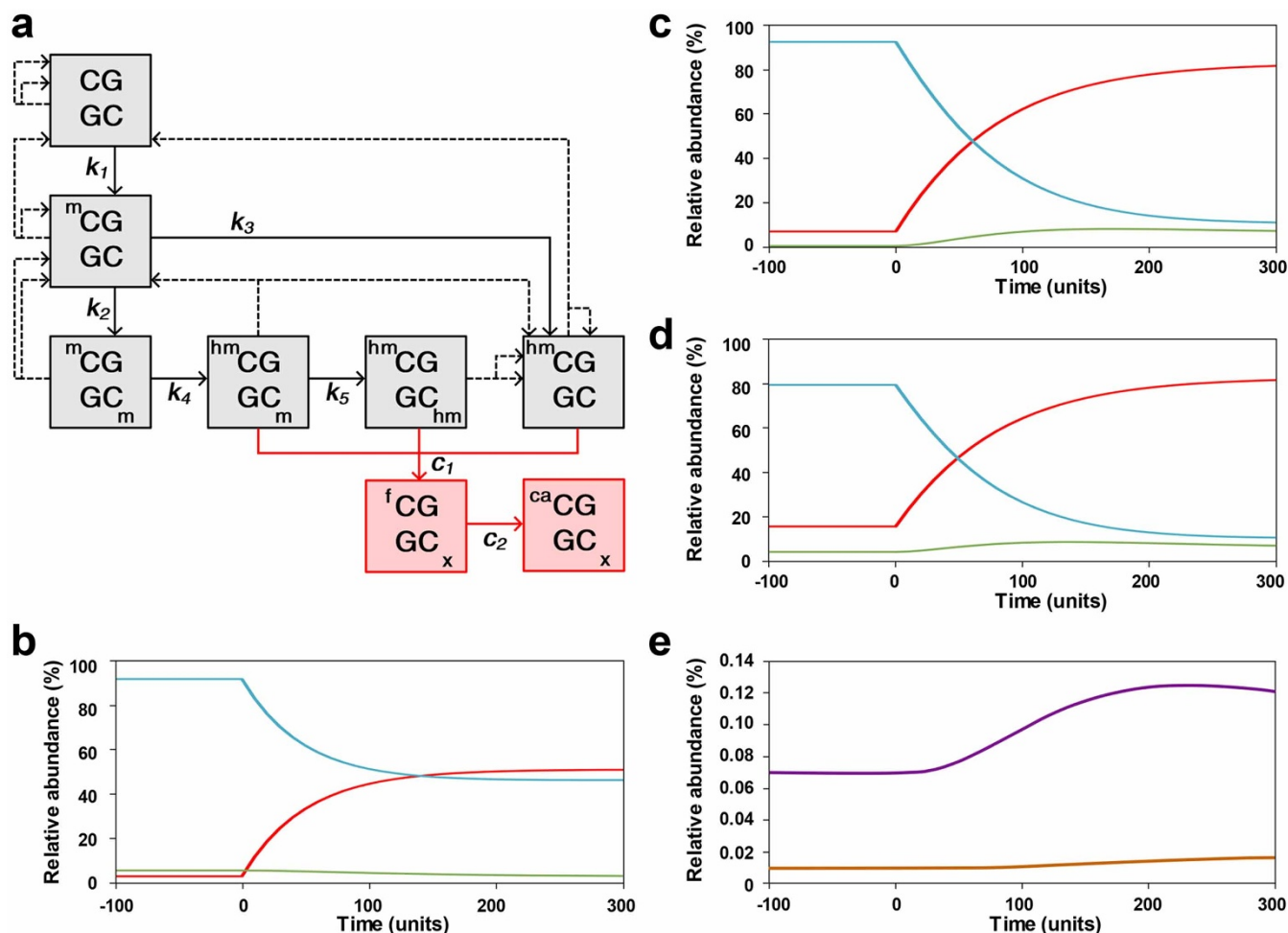
Figure 3 | Mathematical simulation using a multi-compartmental model. (a) A schematic representation of the original six compartmental model components (black) and the extended model components (red). Solid lines indicate epigenetic modification by enzymes. Broken lines indicate the effects of cell division. The effects of DAC treatment (at time = 0) in machina on the relative abundance of unmethylated (red), methylated (blue), and hydroxymethylated (green) CpGs (b) in cells with non-selective TET; (c) in cells with TET proteins which are intrinsically fully selective for hemimethylated CpG dinucleotides; (d) in cells with TET partially selective (6-fold) for hemimethylated CpG dinucleotides; (e) and in cells with TET partially selective for hemimethylated CpG dinucleotides demonstrating the effect on abundance of 5fC (purple) and 5caC (brown).
