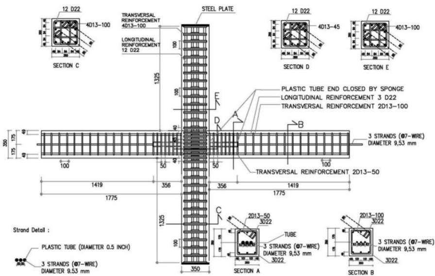
Figure 1 Specimen BCS-I-1B-33.8.
