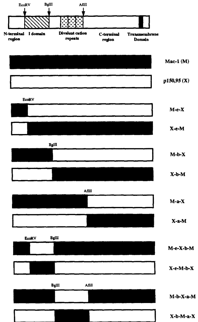
Figure 1. Schematic representation of the leukocyte integrin α chain and Mac-1/p150,95 chimeras. Restriction sites (e, EcoRV; b, BglII; a, AflII) that facilitated reciprocal exchanges are indicated with arrows or in the name of each chimera.
