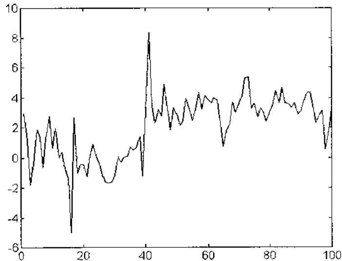
Figure 2. Plot of a simulated AR(1) series with three additive outliers at t = 16, 17, 41 and a level shift at t = 40 .
