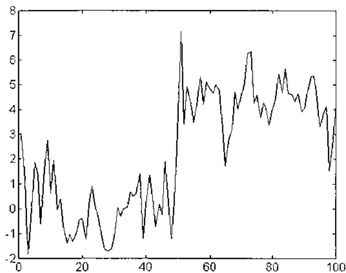
Figure 1. Plot of a simulated AR(1) series with a level shift at t = 50 and an additive outlier at t = 51 .
