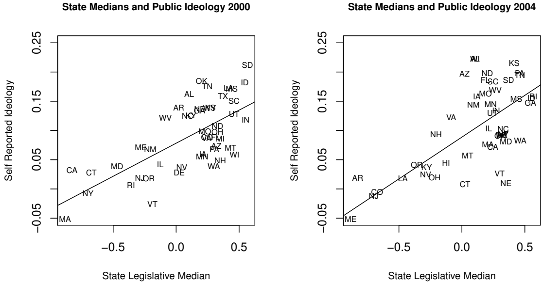
Figure 11: Scatterplot of pooled state legislative medians ( x -axis) against 2000 and 2004 Annenberg mean self-reported ideology ( y -axis). Line is best fit.
