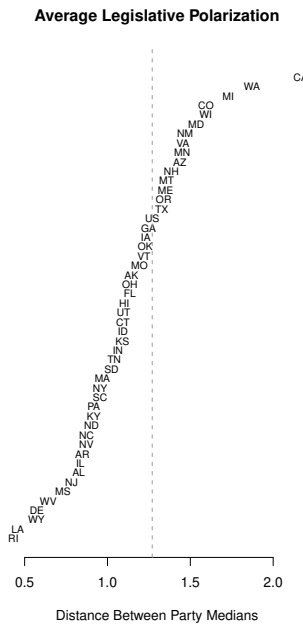
Figure 14: Plot of mean levels of state legislative polarization (measured by distance between party medians) over the full time period available for each state, averaged between both chambers. Dotted line represents average of U.S. Congress polarization for comparison.
