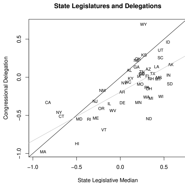
Figure 7: Scatterplot of pooled state legislative medians ( x -axis) against pooled state congressional delegation medians ( y -axis). Dark line is 45 degrees, representing equality of state legislative and state delegation medians. Gray line is best fit.
