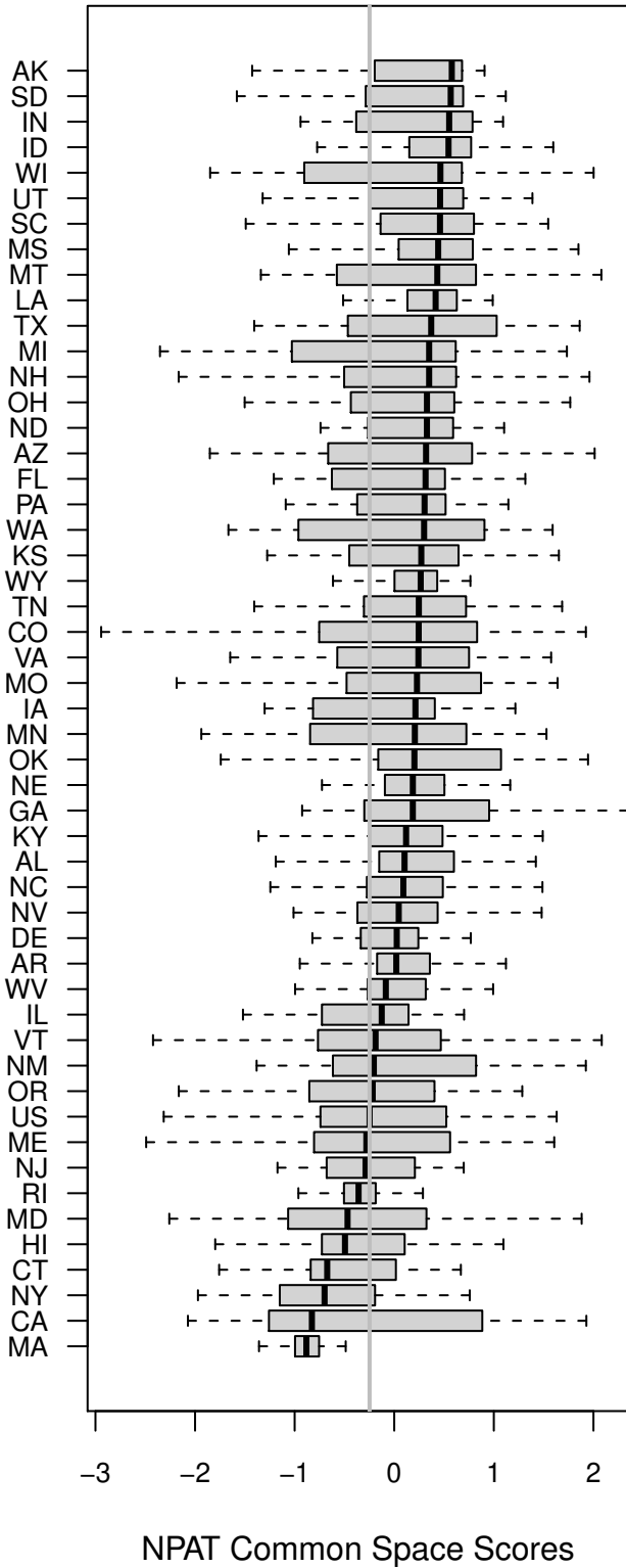
Figure 6: Estimated NPAT common space scores for state legislatures compared with scores for the US Congress, 1996-2006. Left plot pools both parties, while the right plot separates them. Vertical line are drawn at the pooled Congressional median, overall and by party.
