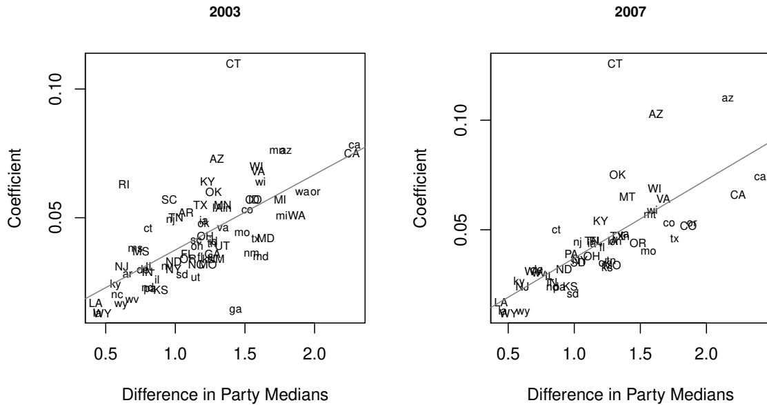
Figure 17: Scatterplot of slope coefficients from repeated cross sectional regressions (“superplot”), plotted against state legislative chamber polarization (measured as the difference in party medians), for 2003 and 2007. Uppercase states are upper chambers, lowercase states are lower chambers.
