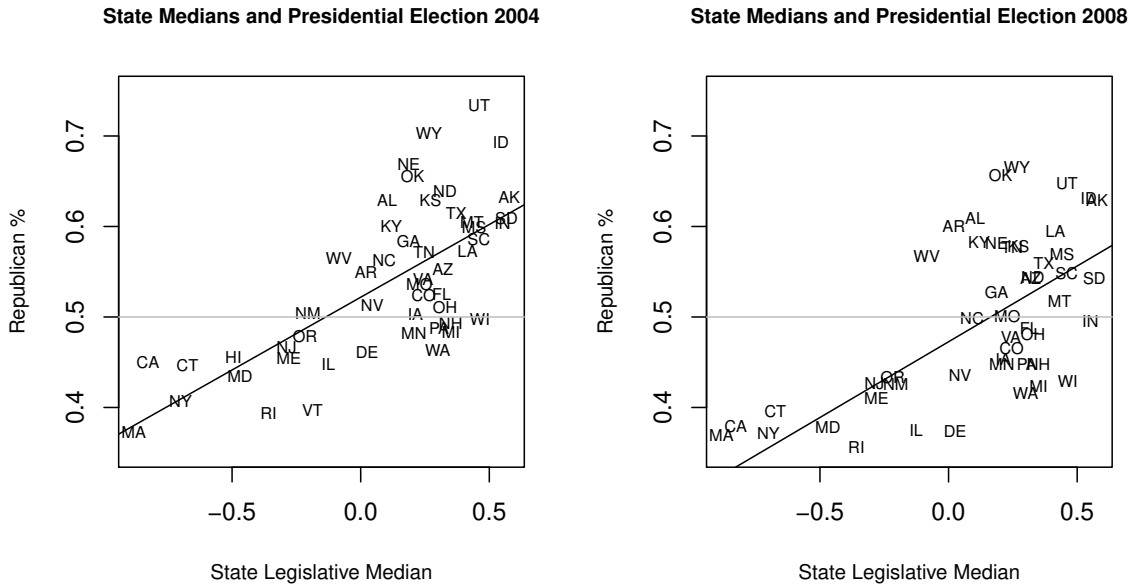
Figure 12: Scatterplot of pooled state legislative medians ( x -axis) against 2004 presidential election results ( y -axis). Line is best fit.
