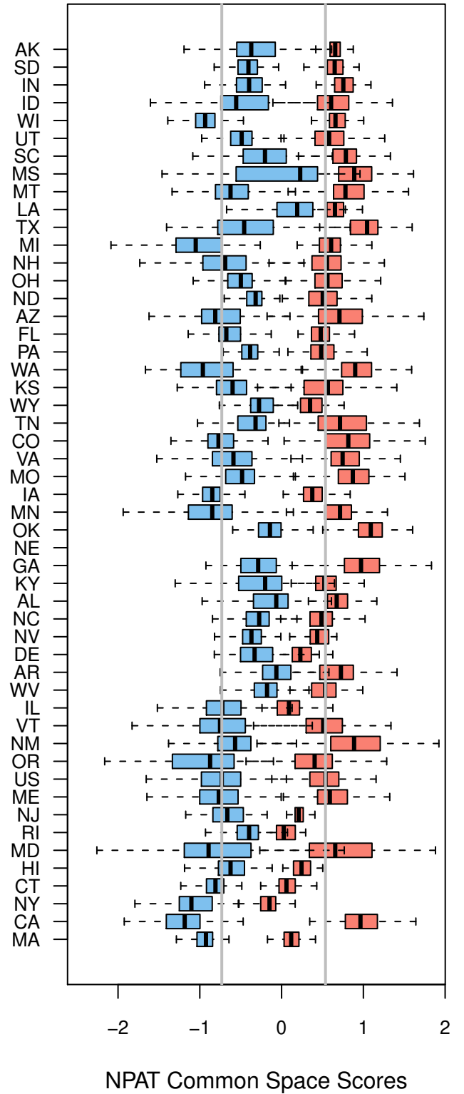
Figure 6: Estimated NPAT common space scores for state legislatures compared with scores for the US Congress, 1996-2006. Left plot pools both parties, while the right plot separates them. Vertical line are drawn at the pooled Congressional median, overall and by party.
