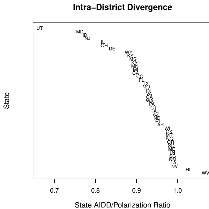
Figure 18: Ratio of Divergence to Polarization by State.
