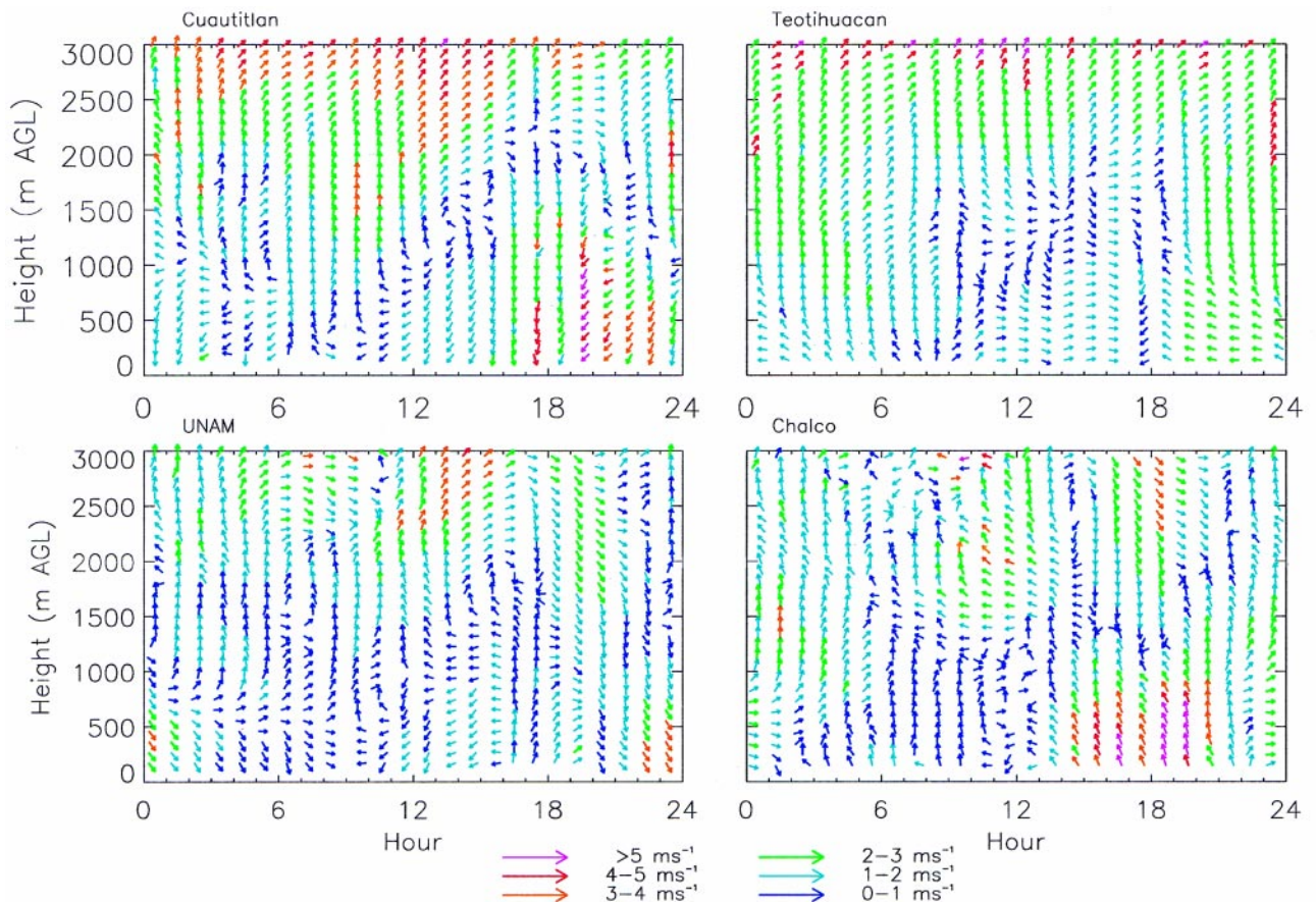
FIG. 9. Radar wind profiles at Cuautitlan, Teotihuacan, UNAM, and Chalco averaged over days with weak synoptic forcing during the IMADA-AVER experiment.
