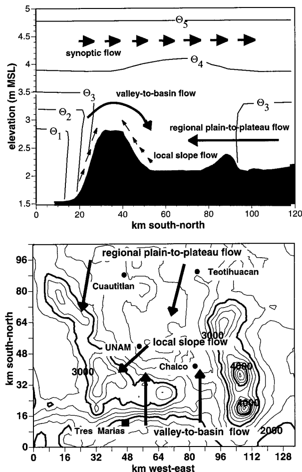
FIG. 3. Schematic diagram showing hypothesized daytime flow patterns affecting the Mexico City basin. (top) Vertical cross section, representative potential temperature contours are shown; (bottom) horizontal cross section, elevations are in meters.
