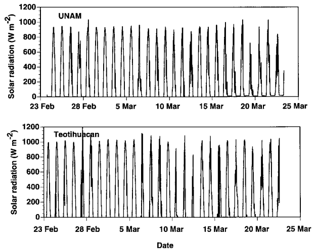
FIG. 6. Solar radiation measured at the Teotihuacan and UNAM sites during the 1997 experiment.
