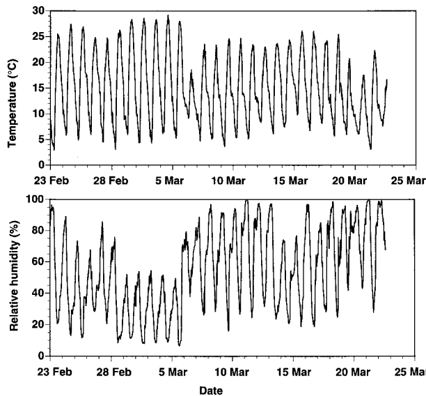
FIG. 5. Near-surface (2 m AGL) temperature and relative humidity time series measured at Teotihuacan during the 1997 experimental period.
