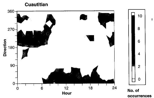
FIG. 11. Distribution of wind vectors at Cuautitlan (28 February–17 March) at 25 m AGL derived from sodar measurements during the 1997 experiment. Each occurrence represents a period of 1 h.
