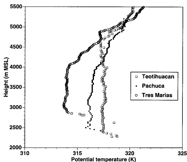
FIG. 8. Potential temperature profiles at approximately 1630 LST at Teotihuacan, Tres Marias, and Pachuca on 11 March 1997.
