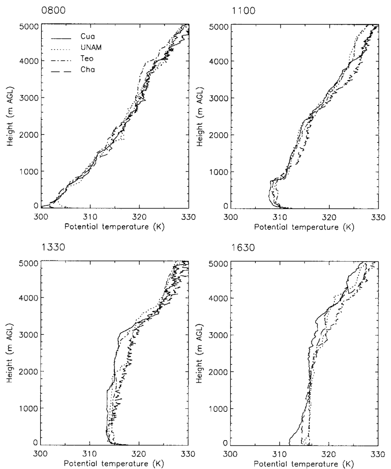
FIG. 7. Potential temperature profiles at the four radar profiling sites at 0800, 1100, 1330, and 1630 LST on 7 March 1997.
