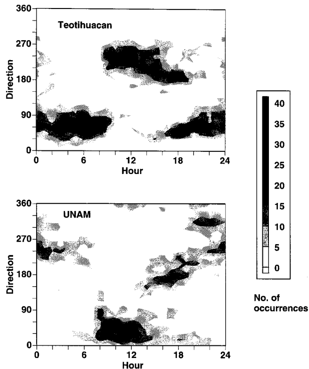
FIG. 10. Distribution of wind directions at 2-m elevation at Teotihuacan (24 February–22 March) and at 10-m elevation at UNAM (25 February–23 March) during the 1997 experiment. Each occurrence represents a period of 15 min.
