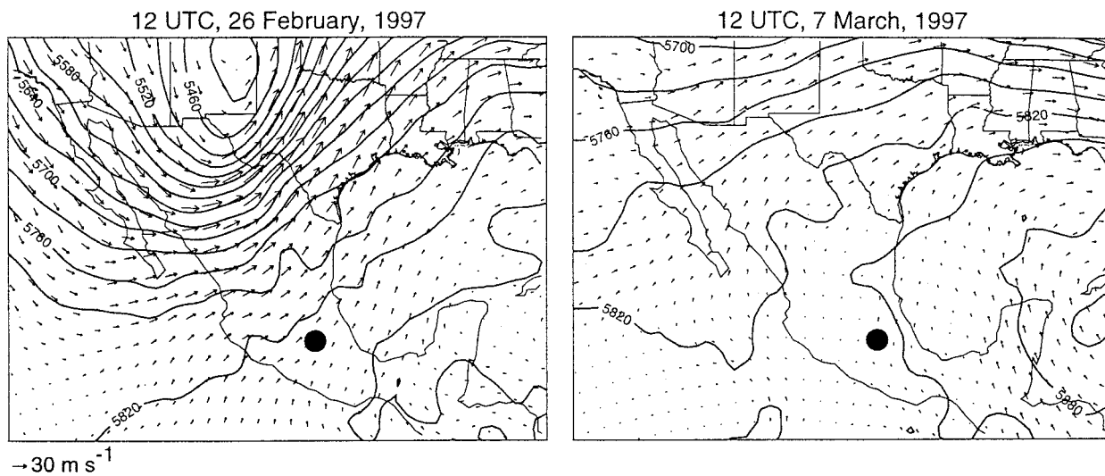
FIG. 4. Maps of the 500-hPa height (m) and wind patterns during two days of the 1997 experiment. The filled circle marks the location of Mexico City.
