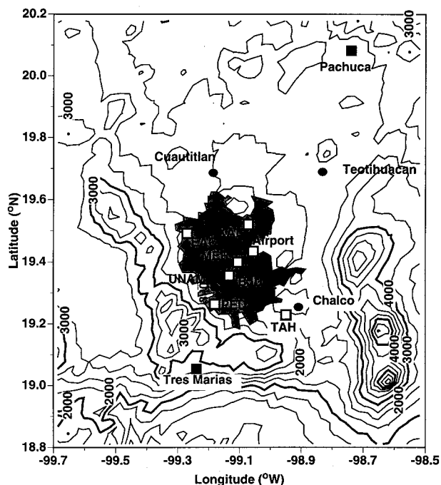
FIG. 1. Topographic map of Mexico City and its surroundings showing locations of the four 915-MHz radar wind profiler sites (filled circles), the Tres Marias radiosonde and Pachuca rawinsonde sites (filled squares), and the airport and six air chemistry monitoring sites (open squares). The gray area marks the approximate bounds of the main Mexico City urban area. Elevations are in meters.
