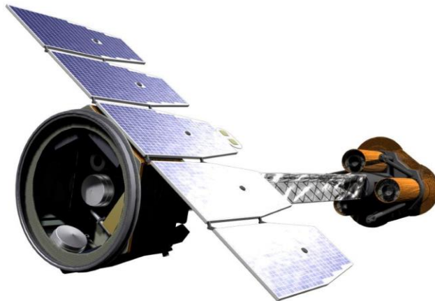
Figure 1. Cartoon mechanical drawing of IXPE as seen along the optical axis from left to right. The spacecraft (S/C) and its solar panels are on the left and the rear of the three telescopes assemblies are on the right. The overall length from aft of the S/C to the front of the optics is approximately 5-m.
