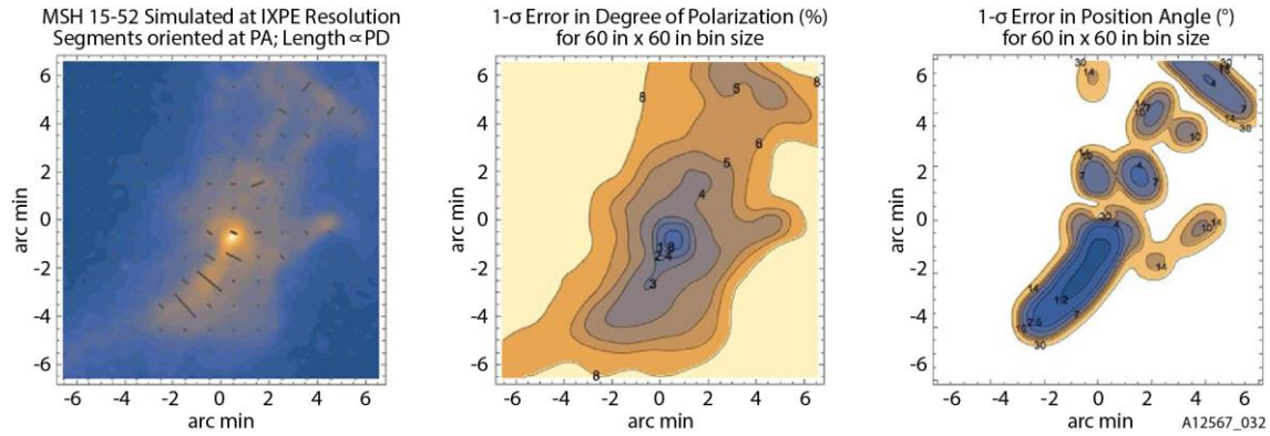
Figure 8 Simulated IXPE polarimetric imaging of the PWNe MSH 15-52 and pulsar B1598-58. Left panel shows the intensity image with superposed polarization model; center, contour map of the uncertainty in the degree of polarization; and right, contour map of the uncertainty in the position angle. Computed errors are for 60'' \times 60'' bins and a long exposure.
