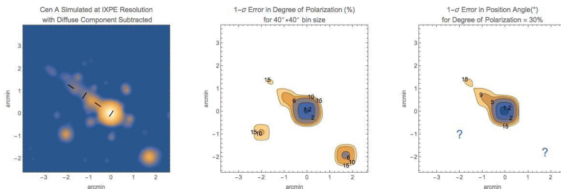
Figure 6. Simulated IXPE polarimetric imaging of the jet in the AGN Cen A. Left: the intensity image with superposed polarization model; center: contour map of the polarization statistical error in polarization degree; and right: contour map of the uncertainties in the position angle. Errors are for 40''×40'' bins and a long exposure.
