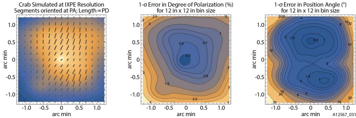
Figure 6. Simulated IXPE polarimetric imaging of the Crab PWNe and pulsar. Left panel shows the intensity image with superposed polarization model; center, contour map the polarization; and right, contour map of the position angle. Computed errors are for 12'' \times 12'' bins and a short exposure.
