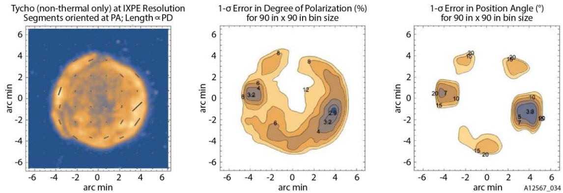
Figure 10. Simulated IXPE polarimetric imaging of the SNR Tycho. Left panel shows the intensity image with superposed polarization model; center, contour map of the uncertainties in the degree of polarization; and right, contour map of the uncertainties in the position angle. Computed errors are for 90'' \times 90'' bins and a long exposure.
