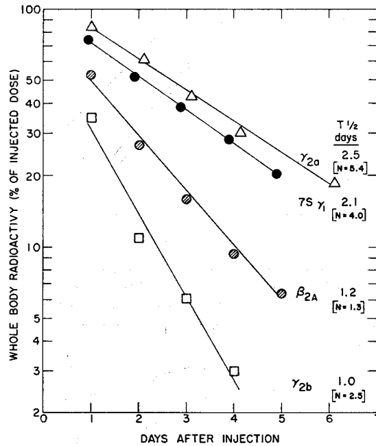
FIG. 5. Catabolism of immunoglobulins, \gamma_{2a} , \gamma_{2b} , 7S \gamma_1 and \gamma_{1A} ( \beta_{2A} ) in mice bearing \gamma_{2a} myeloma protein. The catabolic curves of I^{131} -labeled \gamma_{2a} -, \gamma_{2b} -, 7S \gamma_1 -, and \beta_{2A} -globulins in a group of mice bearing plasma cell tumor Adj.PC-5-producing \gamma_{2a} -myeloma protein are indicated. The T \frac{1}{2} values for the catabolism of each immunoglobulin in normal mice (N) is given in brackets.
