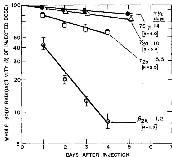
FIG. 4. Catabolism of immunoglobulins, \gamma_{2a} , \gamma_{2b} , 7S \gamma_1 , and \gamma_1A(\beta_{2A}) in low pathogen (CVN-LP) mice. Catabolic decay curves of the radioiodine-labeled immunoglobulins in mice with subnormal numbers of intestinal microorganisms (CVN-LP) are shown. The T_{1/2} values for the catabolism of \gamma_{2a} -, \gamma_{2b} -, 7S \gamma_1 -, and \beta_{2A} -globulins in normal mice (N) are given in brackets below the data obtained in this experiment with low pathogen mice.
