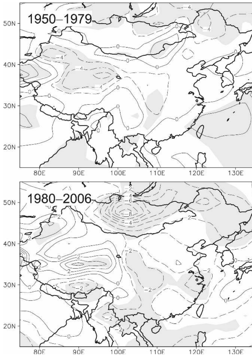
FIG. 7. As in Fig. 6, but for the 850-hPa RH [% (10 yr) -1 ] obtained by NCEP-NCAR reanalysis data. Values significant at the 95% level are shaded.
