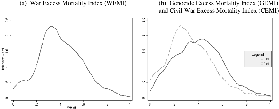
Figure 3: kernel density of the excess mortality indices
