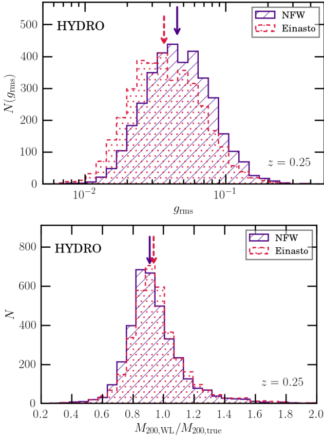
Figure 10. The top panel shows the goodness of fit for the best fit NFW (purple, diagonal hatching) and Einasto (pink, dotted hatching) profiles to the reduced tangential shear profiles of clusters in the HYDRO simulations with M_{200} \geq 10^{14} h^{-1} M_{\odot} at z = 0.25 . The bottom panel shows masses inferred from these fits in units of the true mass. As in 3D, Einasto profiles provide a better fit to the density profiles of clusters and on average provide slightly better estimates of cluster masses.
