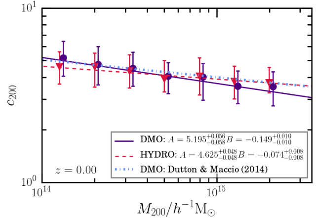
Figure 7. The mass dependence of cluster concentration for the total matter distribution in relaxed BAHAMAS and MACSIS HYDRO (red triangles) and DMO (purple circles) clusters at two different redshifts. Concentrations are obtained by fitting NFW profiles to the total matter density profiles of clusters over the radial range 0.05 \leq r/R_{\text{vir}} \leq 1 . Markers show the median concentrations in mass bins, with error bars indicating the 16th to 84 percentiles. The lines are fits that are obtained by bootstrap resampling a least squares fit of Equation 7 to individual clusters. The concentration-mass relation from Dutton & Macciò (2014) is shown in light blue. DMO clusters have higher concentrations at low masses and exhibit a stronger mass dependence.
