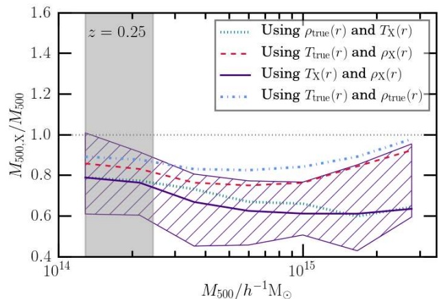
Figure 14. The ratio of X-ray mass to true mass when using the mass weighted temperature T_{\text{true}}(r) profile and the true gas density profile \rho_{\text{true}}(r) (line blue dot-dashed line) as compared to the bias when using the X-ray temperature profile, T_X(r) and the X-ray density profile \rho_X(r) (solid purple line). The hatched region shows the scatter in the bias obtained when using X-ray observables. The shaded grey region shows the mass range where the MACSIS and BAHAMAS simulations overlap. Masses obtained from X-ray observables are consistently lower, with the X-ray temperature providing the largest contribution (some percentage here) to the mass bias.
