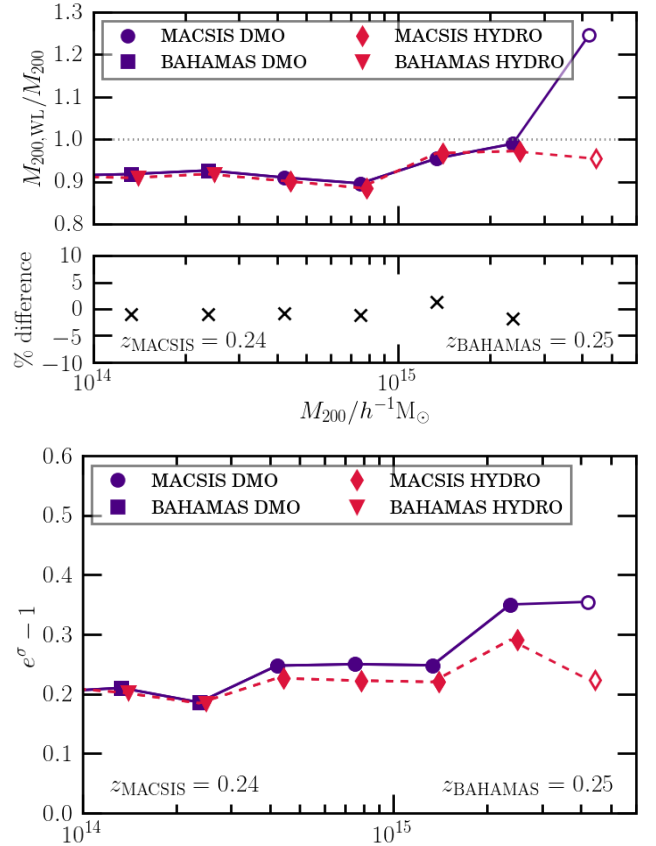
Figure 11. The top panel shows the median ratio of the weak lensing mass to the true mass in mass bins obtained by fitting NFW profiles to reduced tangential shear maps for the DMO (purple solid line) and HYDRO (pink dashed line) simulations as a function of mass. Circles and diamonds (squares and triangles) are used to indicate results from the MACSIS (BAHAMAS) simulations. Markers are offset horizontally for clarity. The unfilled markers represent bins containing fewer than 10 projections. The percentage difference between the DMO and HYDRO result is shown in the middle panel. The bottom panel shows the scatter in the bias as a function of mass, where \sigma is the standard deviation.
