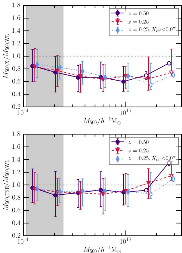
Figure 13. The dependence of the ratio of the X-ray hydrostatic mass to the mass inferred from weak lensing, M_{500,X}/M_{500,WL} , on the true mass of the cluster at z = 0.25, 0.5 . The top panel shows hydrostatic masses derived using spectroscopic temperatures and densities. The bottom panel shows hydrostatic masses derived using true temperatures and densities. Weak lensing masses and hydrostatic masses are calculated independently. The shaded grey region shows the mass range where the MACSIS and BAHAMAS simulations overlap. Excluding the highest mass bin (which contains fewer than 10 clusters), the ratio decreases as a function of mass when using spectroscopic values. The mass bias is independent of redshift. Selecting relaxed clusters (clusters with X_{\text{off}} < 0.07 ) has no significant effect on the bias. Weak lensing masses were obtained by taking one random projection of each cluster. The markers are offset horizontally for clarity.
