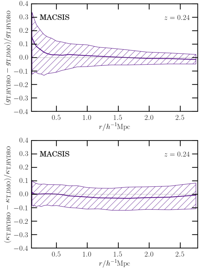
Figure 9. In the top panel the solid purple line is the median fractional difference in the reduced tangential shear profiles, g_T(r) of matched clusters in the DMO and HYDRO MACSIS simulations at z = 0.24 . The hatched purple region shows the 16th and 84th percentiles. The bottom panel shows the fractional difference in the convergence profiles of matched haloes at the same redshift. Baryons have a stronger impact in the central regions of the reduced shear profile than is apparent in the convergence profile.
