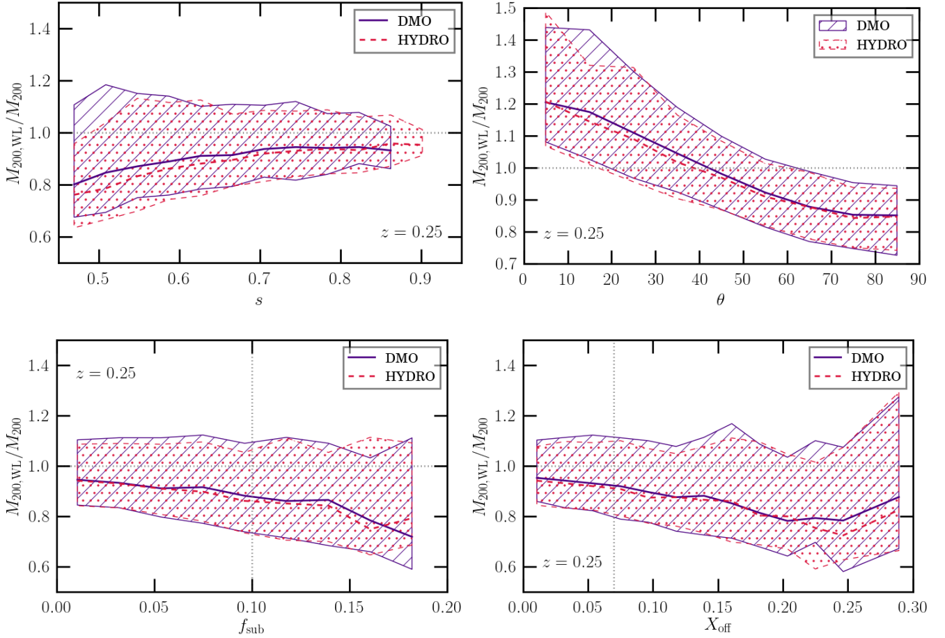
Figure 12. The dependence of the ratio of the weak lensing mass to the true mass, M_{200,WL}/M_{200} , on cluster sphericity, s , alignment, \theta , substructure fraction, f_{\text{sub}} , and centre of mass offset, X_{\text{off}} , at z = 0.25 for both the DMO (purple, diagonal hatching) and HYDRO (pink, dotted hatching) simulations. The solid lines indicate median values and the hatching represents the 1\sigma percentiles. Vertical dashed lines in the bottom panels indicate thresholds used to define relaxed clusters. For alignment, \theta = 90^\circ indicates a cluster with its principal axis perpendicular to the line of sight and \theta = 0^\circ indicates a cluster with its principal axis parallel to the line of sight.
