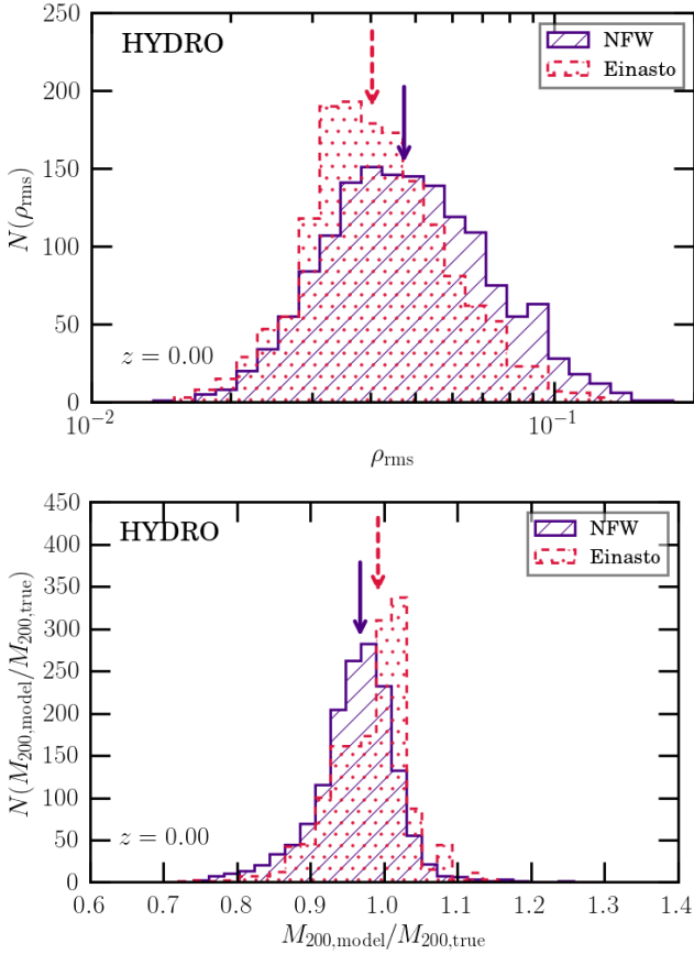
Figure 6. The top panel shows the goodness of fit for NFW (purple, diagonal hatching) and Einasto (pink, dotted hatching) fits to clusters in the HYDRO simulations with M_{200} \geq 10^{14} h^{-1} M_{\odot} at z = 0 . The arrows indicate median values for the NFW (purple) and Einasto (pink) models respectively. The bottom panel shows the mass inferred from the best fit NFW and Einasto profiles. Einasto profiles provide a better fit to the density profiles of clusters and on average provide better estimates of cluster masses.
