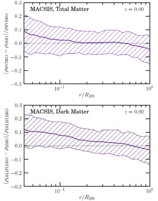
Figure 5. In the top panel the solid purple line is the median fractional difference in the total matter density profiles of matched clusters in the DMO and HYDRO MACSIS simulations at z = 0 . These clusters span the mass range 10^{14.7} \leq M_{200}/h^{-1} M_{\odot} \leq 10^{15.6} . The hatched purple region shows the 16th to 84th percentiles. The bottom panel shows the fractional difference in the dark matter density profiles for matched haloes, where the dark matter density profile in the DMO simulations has been rescaled by a factor of \Omega_{\text{DM}}/\Omega_{\text{m}} , where \Omega_{\text{DM}} is the dark matter fraction and \Omega_{\text{m}} is the total matter fraction.
