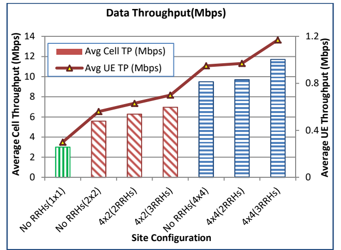
Fig.6 average cell and UE data throughput (Mbps)
