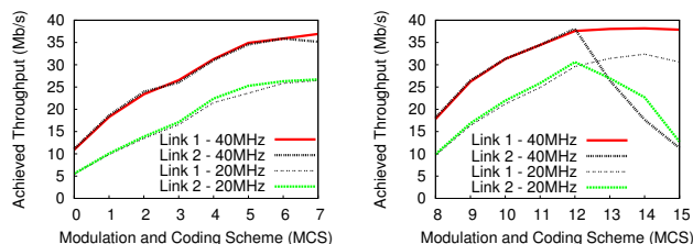
(b) Moderate signal quality (between -43 and -46 dBm)
