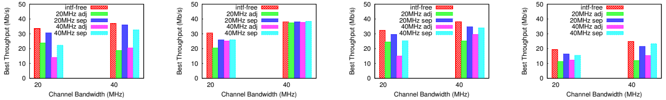
(a) Strong signal quality and strong interferer (b) Moderate signal quality and weak interferer (c) Moderate signal quality and strong interferer (d) Weak signal quality and strong interferer
