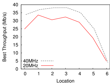
Figure 1: Throughput achieved between single transmitter and receiver pairs at varying locations. The locations are sorted in order of decreasing RSSI.
