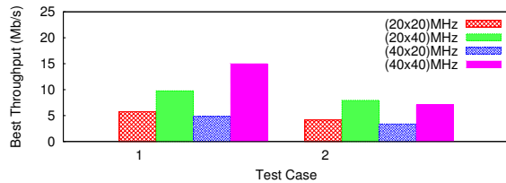
Figure 7: Best throughput for a link (location 1 in Figure 6) suffering from co-channel interference. In Test Case 1, the overlapping transmitter has good link quality to its receiver and operates at MCS 10. In Test Case 2, the overlapping transmitter has poor link quality to its receiver, and thus operates at MCS 0.
