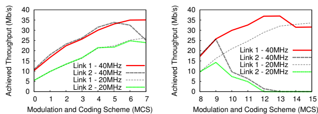
(a) Good signal quality ( > -30 dBm)
