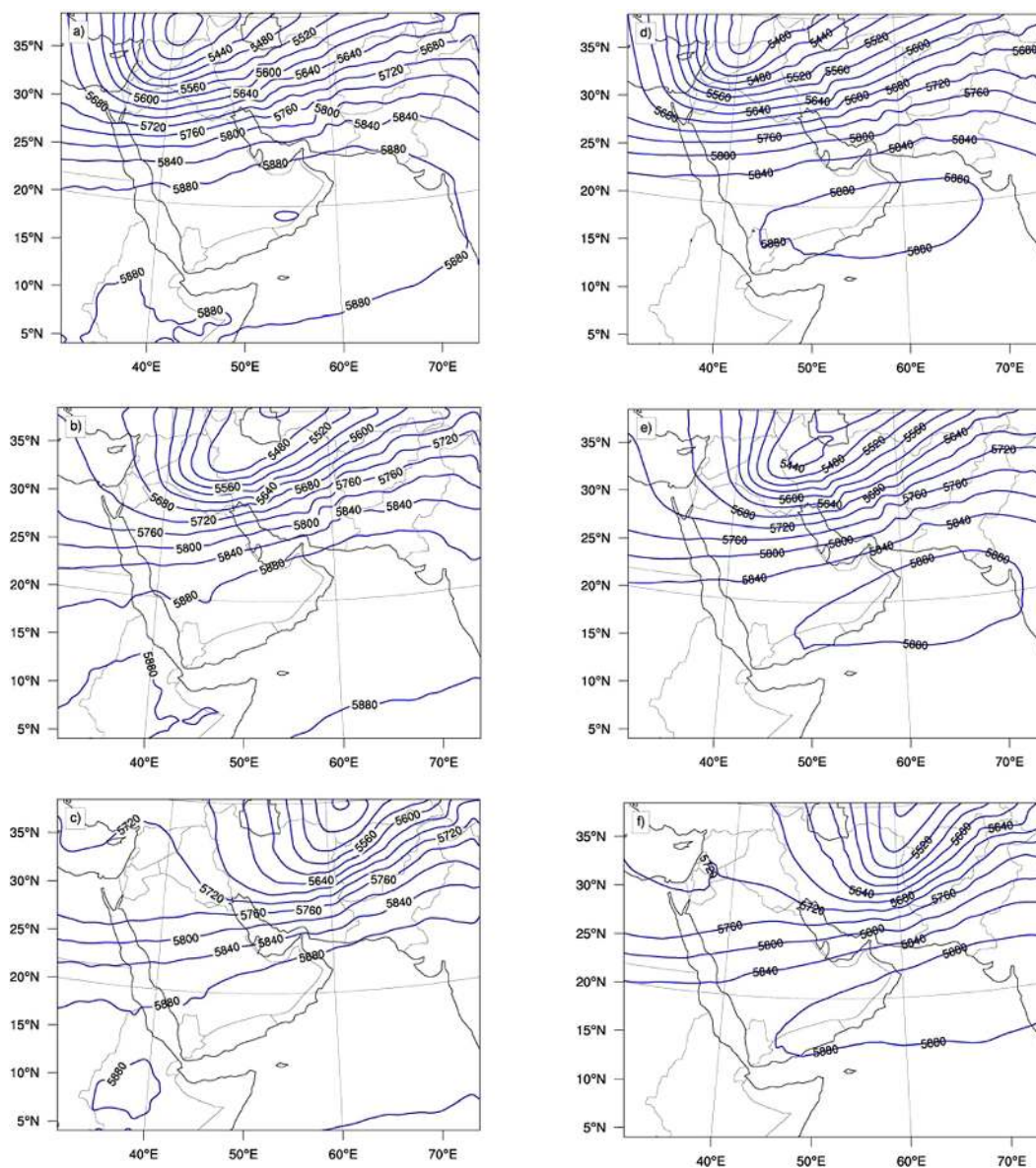
Figure 1. Geopotential height (m) at 500 hPa at 00:00 UTC from WRF–Chem simulations on (a) 17 March, (b) 18 March, and (c) 19 March 2012 and from ERA-Interim reanalysis on (d) 17 March, (e) 18 March, and (f) 19 March 2012.
