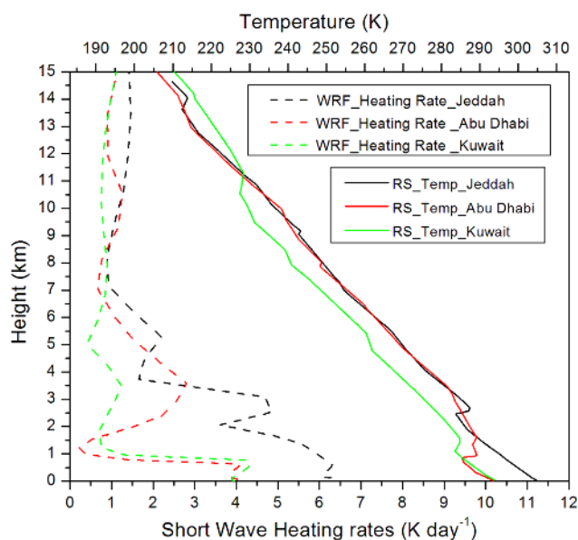
Figure 14. Simulated (dashed lines) solar heating rates profiles in the atmosphere over Jeddah (black), Abu Dhabi (red), and Kuwait (green) sites and radiosounding temperature profiles at the same locations (solid lines) at 12:00 UTC on 19 March 2012.
