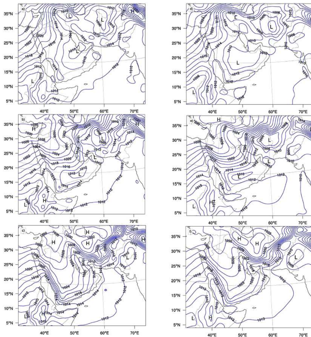
Figure 2. Sea-level pressure (hPa) with H and L markers indicating low and high pressure systems at 00:00 UTC from WRF–Chem simulations on (a) 17 March, (b) 18 March, and (c) 19 March 2012 and from ERA-I reanalysis on (d) 17 March, (e) 18 March, and (f) 19 March 2012.
