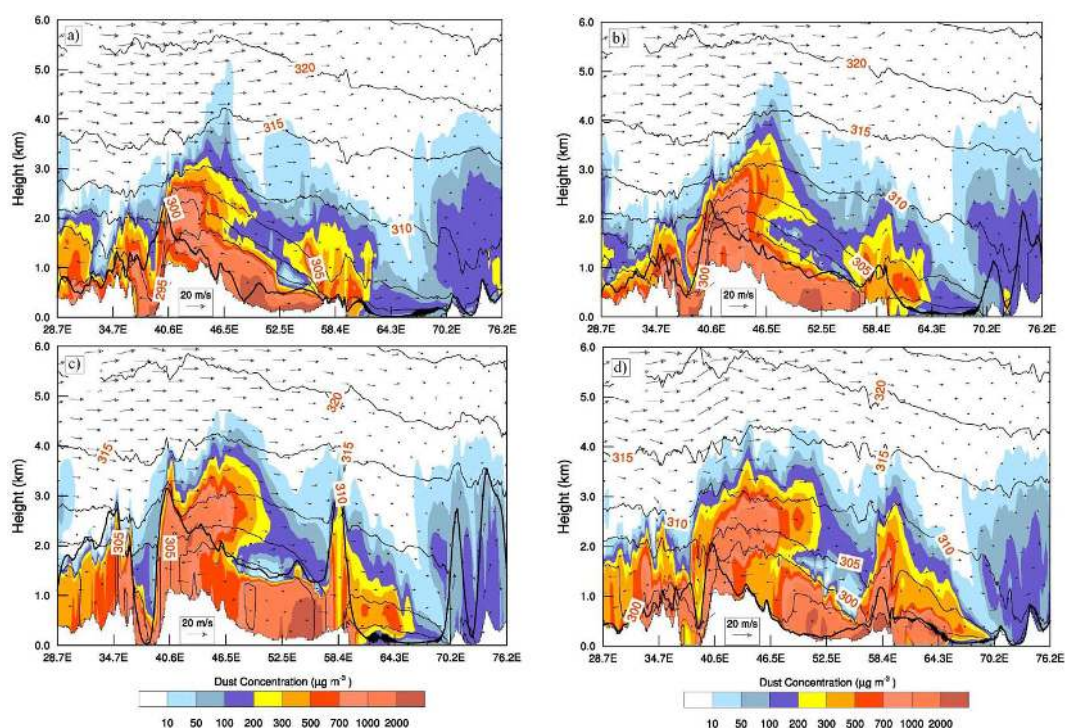
Figure 10. The height longitude cross section along 21.7^\circ N showing dust concentration ( \mu\text{g m}^{-3} , shading) and PBL height (km) shown by the black solid line from WRF-Chem on 19 March 2012 at (a) 00:00 UTC, (b) 06:00 UTC, (c) 12:00 UTC, and (d) 18:00 UTC.
