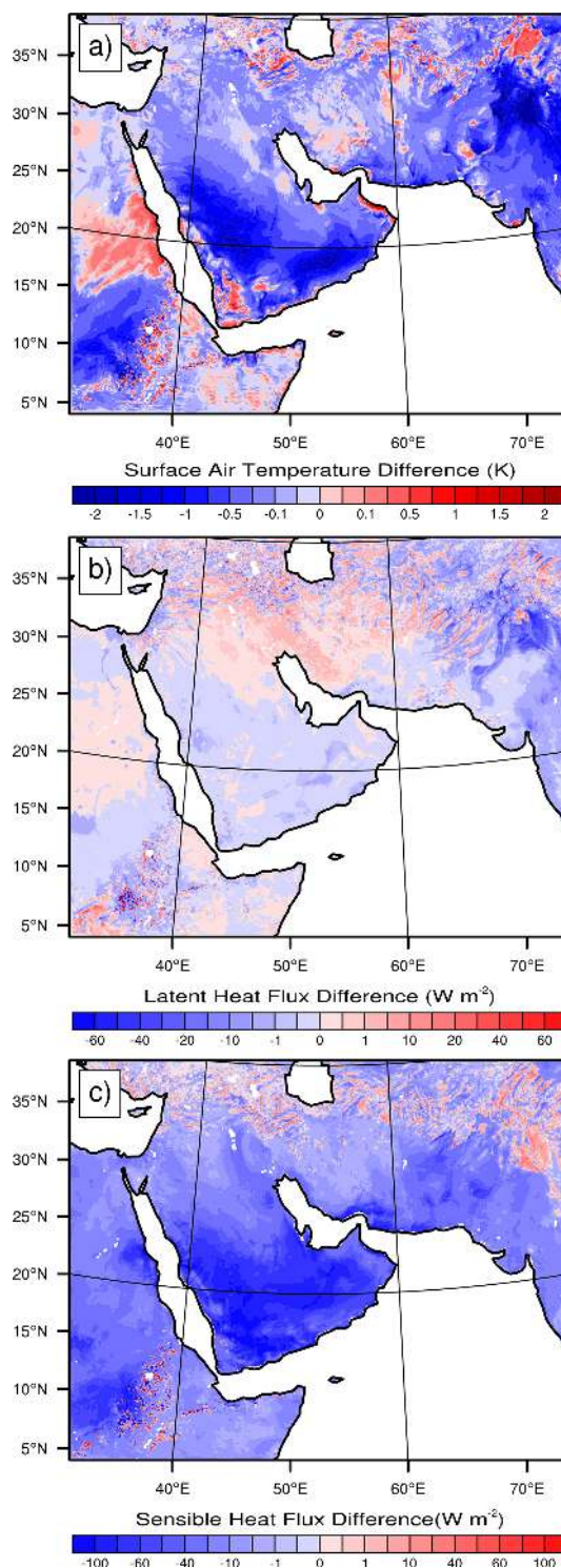
Figure 15. Simulated instantaneous differences in (a) air temperature (K), (b) latent heat flux ( \text{W m}^{-2} ), and (c) sensible heat flux ( \text{W m}^{-2} ) in the runs with and without dust aerosols at 12:00 UTC on 19 March 2012.
