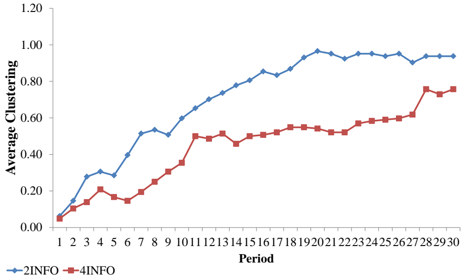
Figure 8b: Average G-clustering by Treatment and Period
