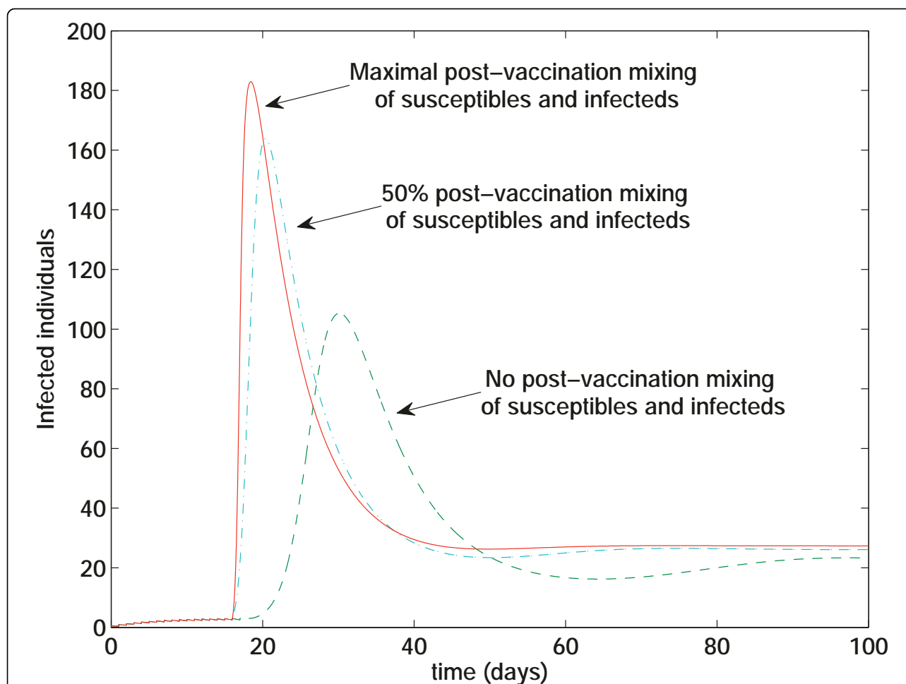
Figure 8 The effect of different post-panic mixing rates Comparison of mixing rates between susceptibles and infected individuals after a vaccinating panic. The more susceptibles mix with infecteds, the earlier the outbreak occurs and the larger the number of infected individuals.
