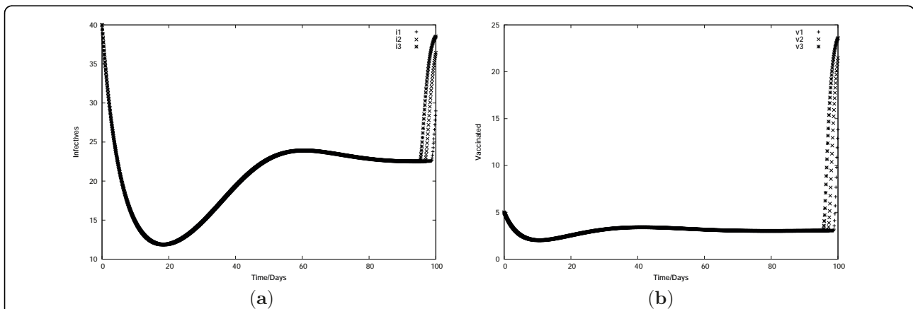
Figure 5 Optimalty effect when the weight constraint for the control varies and media has an adverse effect on the vaccine. Graphs of the optimalty system when media coverage has an adverse effect on the vaccination rate and when the weight constraint for the control population varies. (a) Graph of infectives. (b) Graph of vaccinated individuals. Initial conditions: S(0) = 20.0 , I(0) = 25.0 , V(0) = 50.0 , R(0) = 40.0 . The value of the weights used are (i) B2 = 25.0 corresponds to variables with subscript 1 (++), (ii) B2 = 2500.0 corresponds to variables with subscript 2 (xx), (iii) B2 = 250000.0 corresponds to variables with subscript 3 (**). The value B1 = 0.0025 is kept constant in all three cases.
