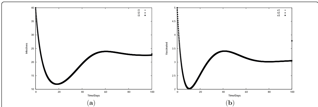
Figure 4 Optimalty effect when the weight constraint for the infected population varies and media has an adverse effect on the vaccine. Graphical representation of the optimalty system when media coverage has an adverse effect on the vaccination rate and when the weight constraint for the infected population varies. (a) Graph of infectives. (b) Graph of vaccinated individuals. Initial conditions: S(0) = 20.0 , I(0) = 25.0 , V(0) = 50.0 , R(0) = 40.0 . The value of the weights used are (i) B1 = 0.0025 corresponds to variables with subscript 1 (++), (ii) B1 = 25.0 corresponds to variables with subscript 2 (xx), (iii) B1 = 250000.0 corresponds to variables with subscript 3 (**). The value B2 = 0.0025 is kept constant in all three cases.
