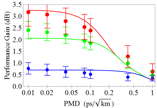
Fig. 2. Influence of PMD on the NLC gain of a 5x32 Gbaud dual polarisation 16QAM Nyquist WDM system over 40*80.17km spans with digital back propagation, showing (dots) simulated results [8] and (solid line) predictions of Eqn 3 for one (blue), three (green) and five (red) channel DBP. 10 fibre realisations were used for PMD studies. Error bars are 2 standard deviations.
