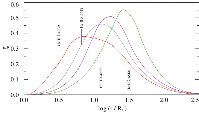
Fig. 4. Normalized \xi(\log r) -plots for several He II emission lines belonging to the model of the star BAT99 7. The model parameters are listed in Table 1. The individual lines are formed many stellar radii above the surface.
