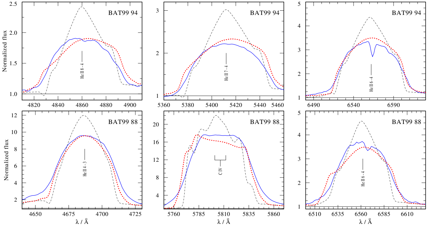
Fig. 7. Zoomed-in sections of Fig. 6 with prominent emission lines of the stars BAT99 94 ( upper panels ) and BAT99 88 ( bottom panels ). The observed spectrum (solid blue line) is compared to the synthetic spectrum calculated with rotation (dotted red line), and without rotation (dashed black line).
