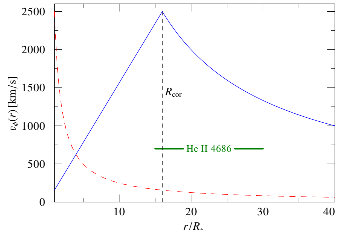
Fig. 5. Equatorial rotational velocity as a function of r . Both curves correspond to v_{\text{cor}} = 2500 \text{ km s}^{-1} . However, the dashed red curve is plotted with R_{\text{cor}} = R_* , while the solid blue curve is plotted with R_{\text{cor}} = 16 R_* . We also denote an estimate of the LFR of the line He II \lambda 4686 , determined by its corresponding \xi plot. Note that the LFR remains unaffected by rotation unless large co-rotation radii are assumed.
