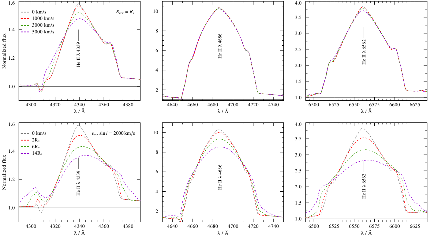
Fig. 3. Effect of the parameters v_{\text{cor}} \sin i and R_{\text{cor}} on prominent synthetic emission lines of BAT99 7. Each of the upper panels depicts, for a constant value R_{\text{cor}} = R_* , the synthetic profile of an emission line calculated with different v_{\text{cor}} \sin i values. The bottom panels show the synthetic profile of the same spectral lines calculated with different R_{\text{cor}} values and with a constant rotational velocity of v_{\text{cor}} \sin i = 2000 \text{ km s}^{-1} .
