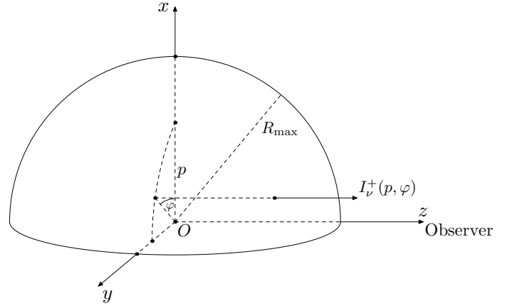
Fig. 2. The coordinate system used for the 3D integration scheme. The integration of the emergent intensities I_\nu^+(p, \varphi) is performed over the impact parameter p and the azimuthal angle \varphi . The z -axis points towards the observer.
