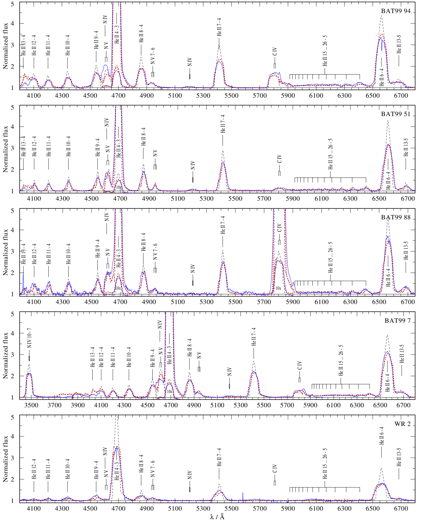
Fig. 6. Comparison between synthetic spectra calculated with rotation (dotted red line), without rotation (dashed black line), and observations (solid blue line) for the five stars analyzed. The synthetic spectra are convolved with a Gaussian of FWHM = 3 \text{ \AA} to account for instrumental broadening.
