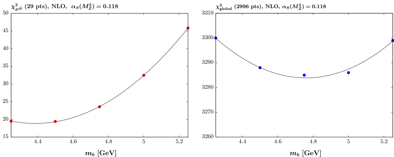
Fig. 5 The quality of the fit versus the quark mass m_b at NLO with \alpha_S(M_Z^2) = 0.118 for (left) the reduced cross section for beauty production \sigma^{bb} for the H1 and ZEUS data and (right) the global fit, not including the beauty data
