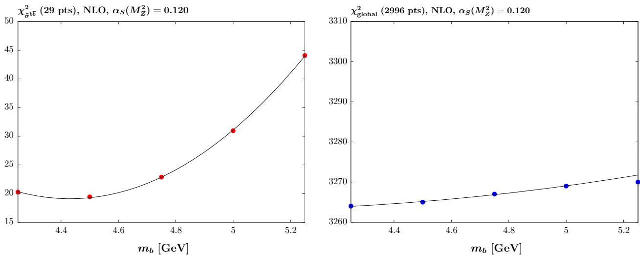
Fig. 4 The quality of the fit versus the quark mass m_b at NLO with \alpha_S(M_Z^2) = 0.120 for (left) the reduced cross section for beauty production \sigma^{bb} for the H1 and ZEUS data and (right) the global fit, not including the beauty data
