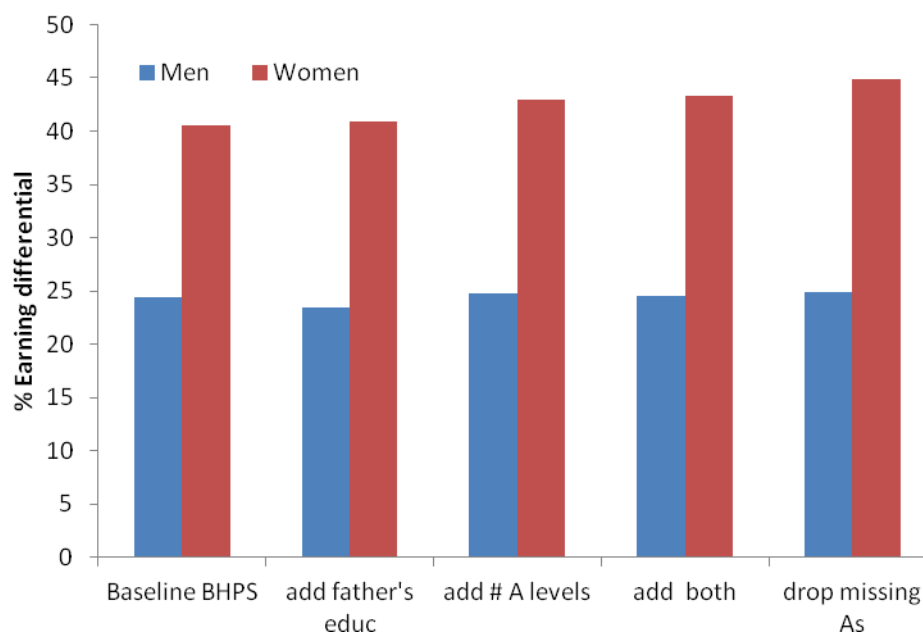
Figure 14 Robustness of BHPS baseline results
