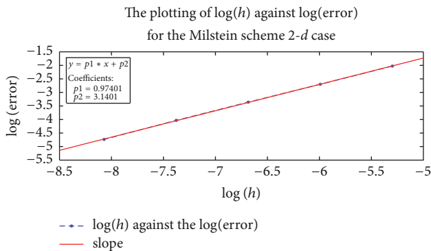
FIGURE 1: Milstein method for the two dimension SDEs.
