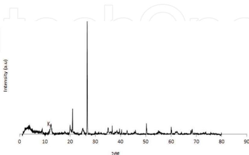
Figure 10. The XRD curve for typical clay.
