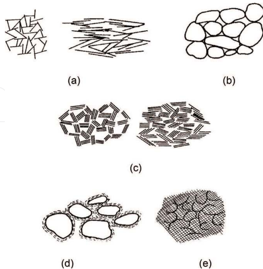
Figure 6. Arrangement of clay particles [11]. (a) Elementary particle arrangements of clay; (b) elementary particle arrangements of sand and silt; (c) clay assemblages; (d) clay coated silt and sand arrangement; (e) not fully defined arrangement.
