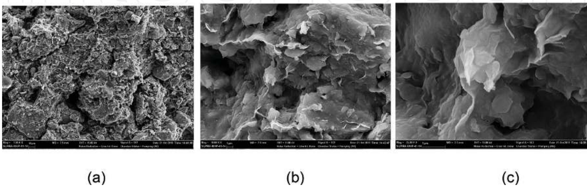
Figure 12. The SEM images of typical clay for different magnification (a. 1000 \times , b. 10,000 \times , c. 35,000 \times ).
