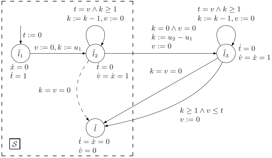
Fig. 5. Translating positive integer slopes
