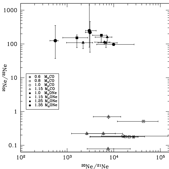
FIG. 6.—Same as Fig. 4, but for 20 Ne/ 21 Ne and 20 Ne/ 22 Ne ratios. [See the electronic edition of the Journal for a color version of this figure.]
