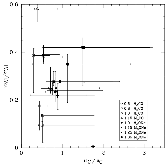
FIG. 7.—Same as Fig. 4, but for 26 Al/ 27 Al and 12 C/ 13 C ratios. [See the electronic edition of the Journal for a color version of this figure.]
