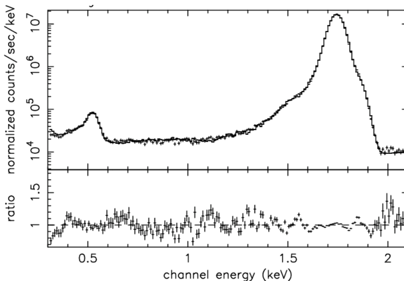
Figure 1. XRT PC mode single pixel event spectrum measured at Leicester from the Si K α and Si K β lines (1.74 and 1.84 keV) with background O K α (0.525 keV) and Bremsstrahlung continuum, together with pre-flight modeled response.
